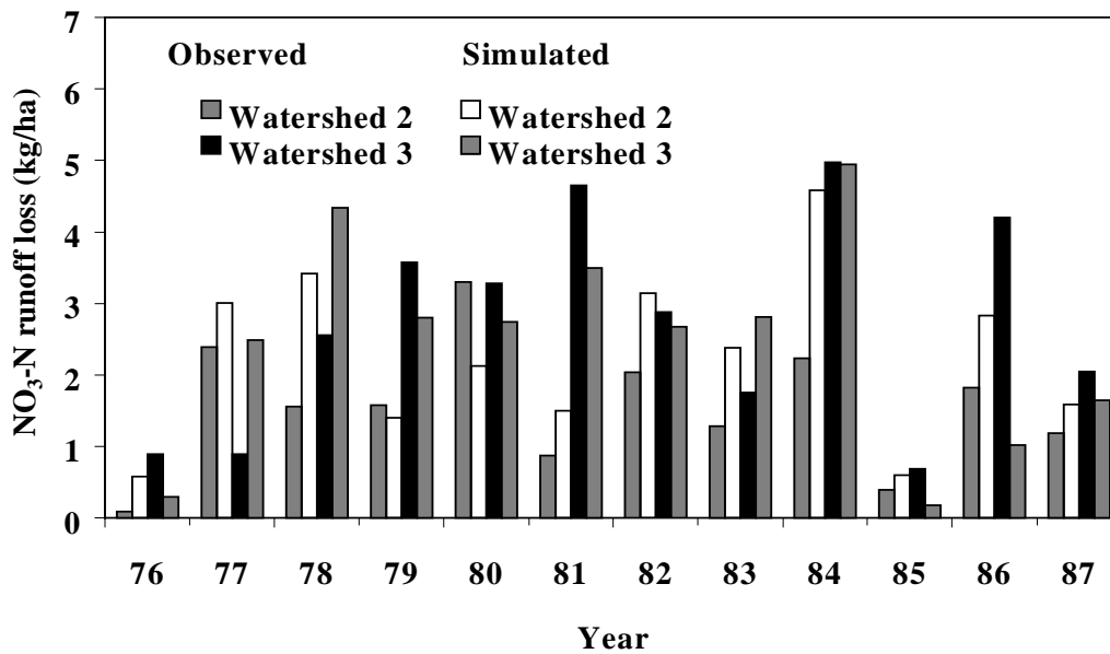
Figure 3. Observed and Simulated Annual NO 3 -N Loss Via Surface Runoff for Watersheds 2 and 3 During the Validation Period. Source: S.W. Chung, P.W. Gassman, L.A. Kramer, J.R. Williams, and R. Gu
