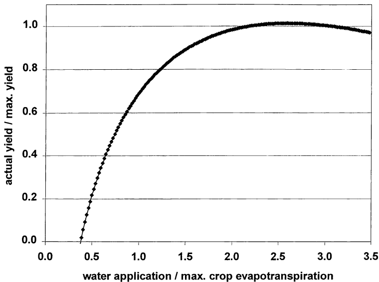
Fig. 2. Crop yield function, crop yield (wheat) vs. water application (CUC = 70, Salinity = 0.7 dS/m).
