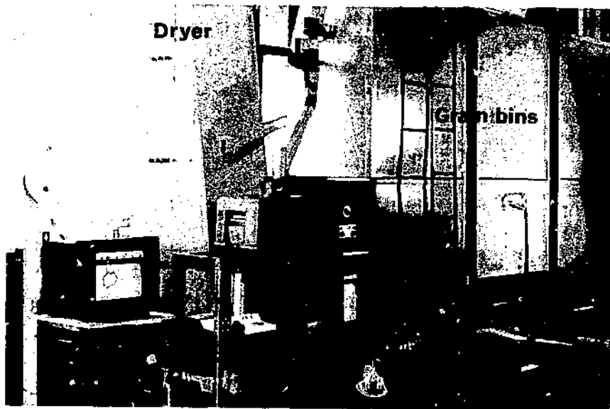
FIGURE 13.—Laboratory dryer and related facilities used to evaluate drying characteristics related to a moisture controller.
