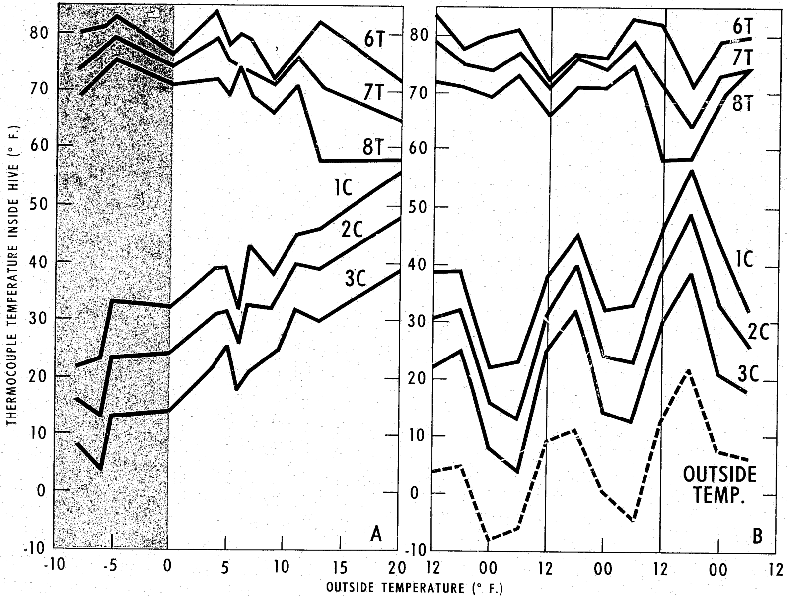
FIGURE 8.—Temperature variation in check colony versus outside temperature. (Thermocouple 8T is three-eighths inch above bottom edge of top body and 1C is one-fourth inch below top edge of center body; others are 1 inch apart in their respective directions.)
