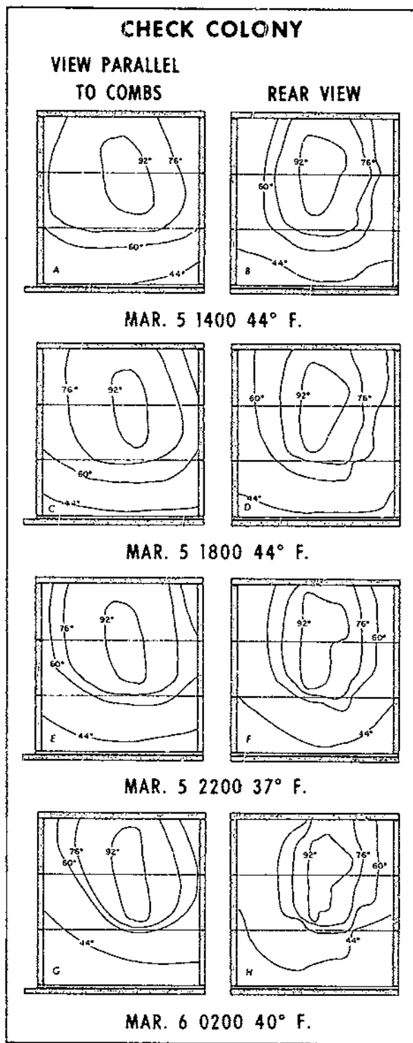
FIGURE 7.—Cluster movement of check colony during day and night with little or no change in outside temperature, showing views parallel to combs and corresponding rear views.
