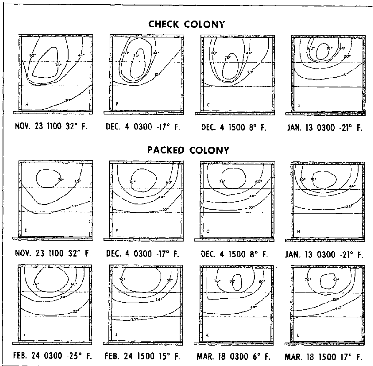
FIGURE 23.—Distribution of isotherms and cluster changes along comb of check and packed colonies in refrigerator at various dates. (Views parallel to combs.)
