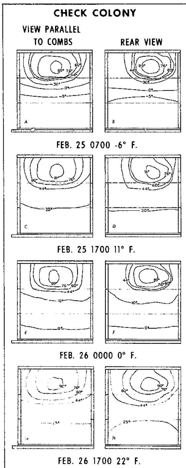
FIGURE 5.—Effect of outside temperature change on isotherms of check colony, showing views parallel to combs and corresponding rear views.
