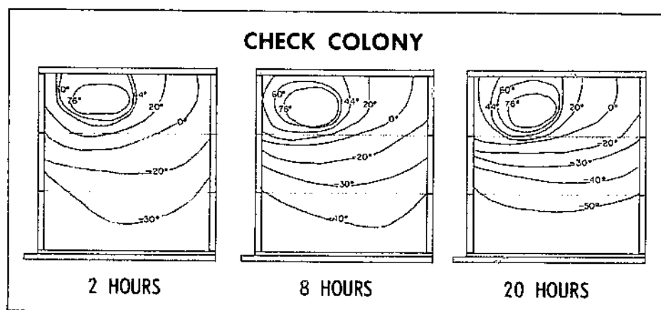
FIGURE 19.—Check colony held at -50° F., showing how hive cooled. Time is in hours after constant temperature was set. (Views parallel to combs.)
