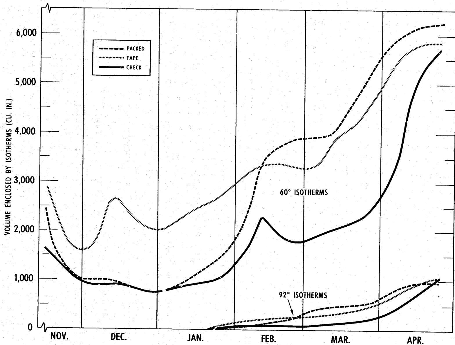
FIGURE 14.—Effect of date on changes in 60° and 92° F. isotherm volumes for each treatment. Each line represents mean of all colonies for that treatment.
