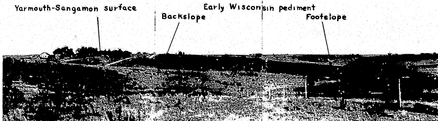
FIGURE 37.—Stepped sequence of topographic levels along interfluvium in South Turkey Creek area. Note nearly level Early Wisconsin pediment footslope and concave backslope that rises to Yarmouth-Sangamon surface. Landscape loess-mantled.
