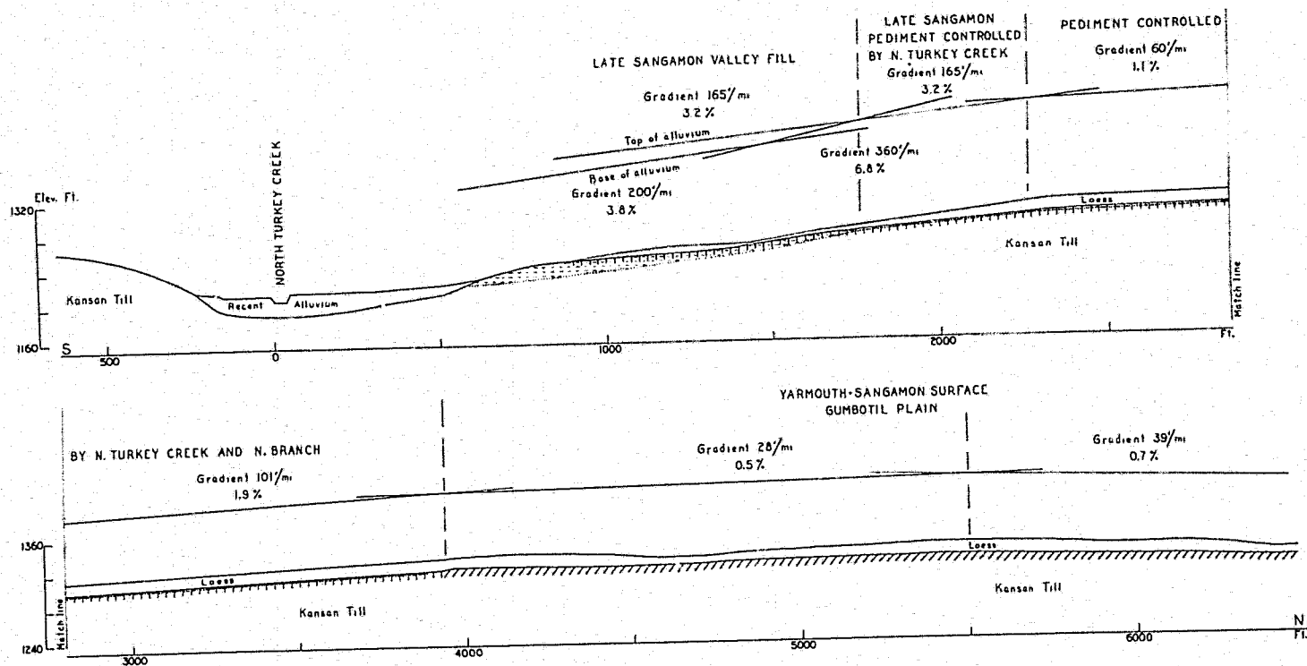
FIGURE 48.—Geomorphic profile along axis of interfluvium north of North Turkey Creek (fig. 45, C-B; pl. IV: D.15, 6.55-B.35, 2.25).
