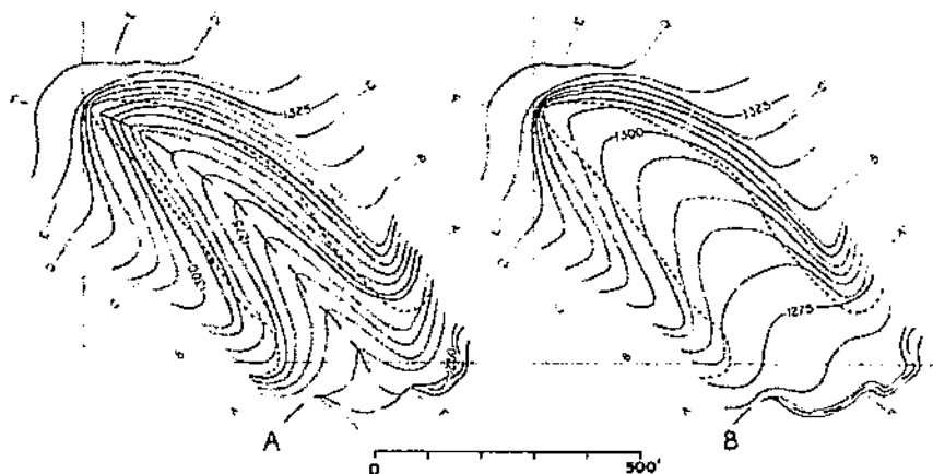
FIGURE 61.—Surface configuration of side-valley waterway after dissection (A) and after fill (B).
