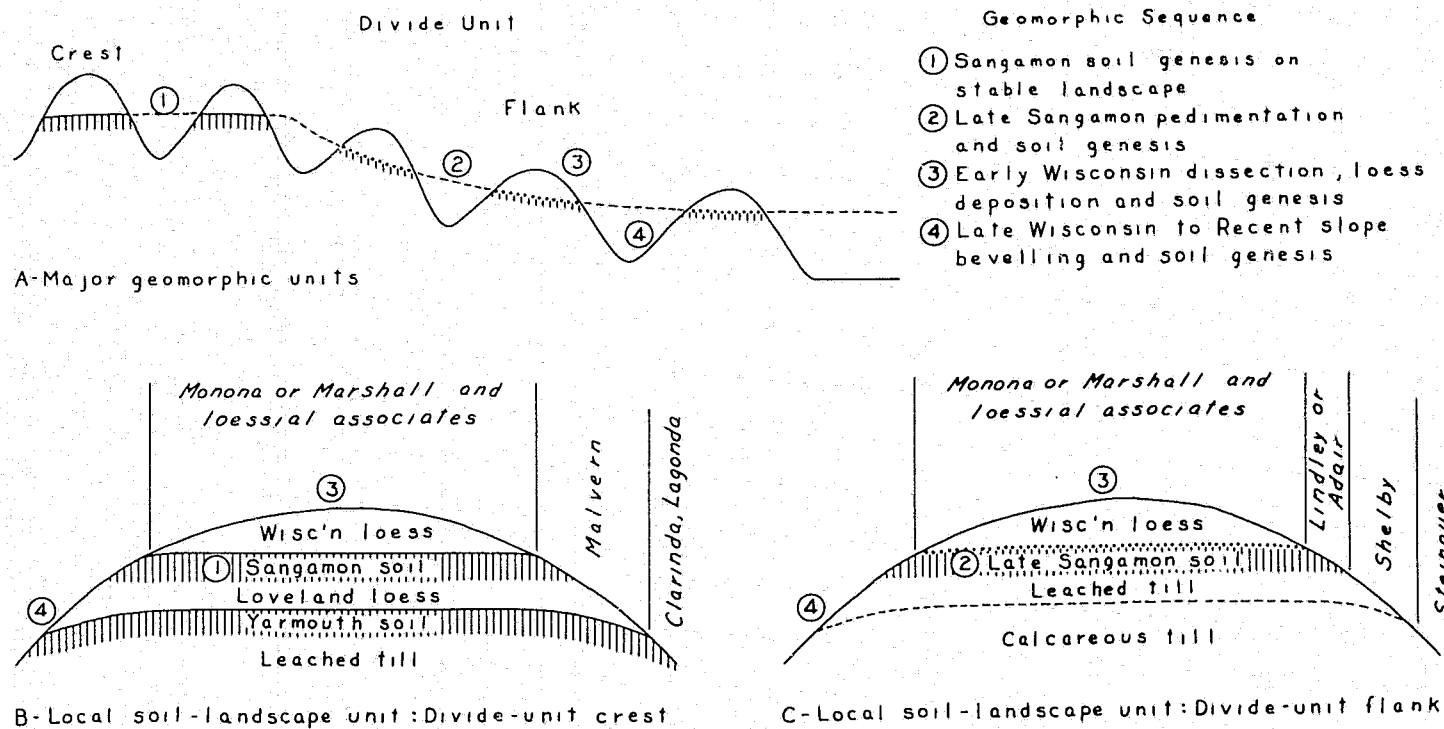
FIGURE 28.—Diagrammatic relationship of geomorphic units and soil geography in western part of traverse.
