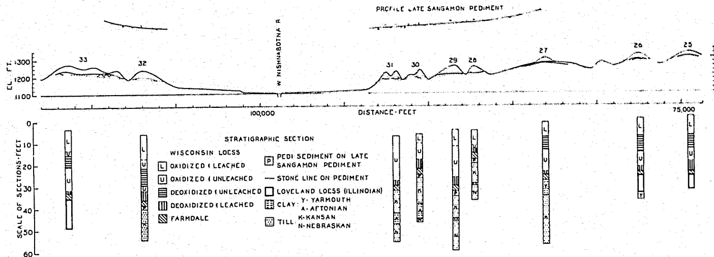
FIGURE 19.—Stratigraphic and geomorphic relationships of Late Sangamon erosion surface flanking West Nishnabotna River, cuts 33 to 25.
