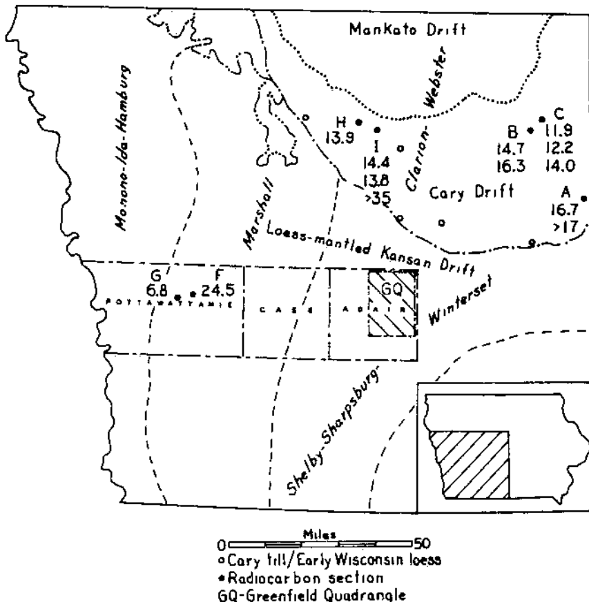
FIGURE 53.—Relationship of Greenfield quadrangle (GQ) to radiocarbon sections of Des Moines lobe, Cary and Mankato drifts. Monona-Ida-Hamburg, Marshall, Shelby, Sharpsburg-Winterset are soil association areas.
