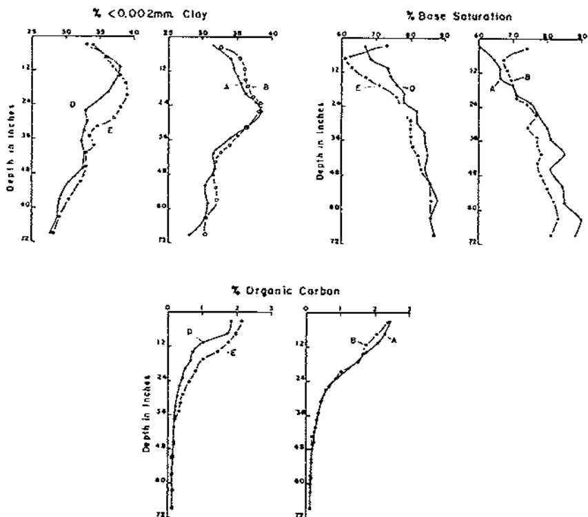
FIGURE 71.—Distribution with depth of clay, percent base saturation, and organic carbon of soils on the Tazewell surface. A and B, unit 12 profiles; D and E, unit 11 profiles.
