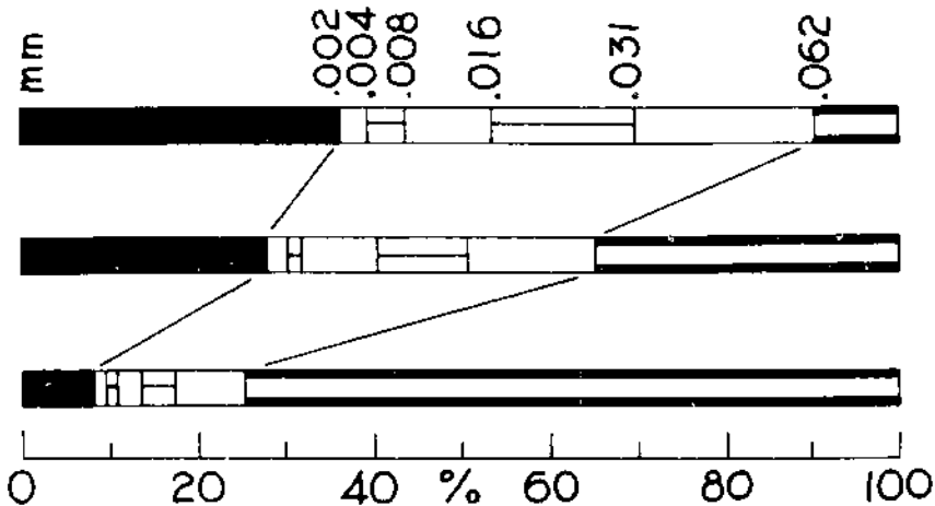
FIGURE 23.—Textures of Late Sangamon alluvium, cut 7.
