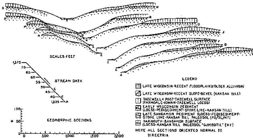
FIGURE 36.—Geomorphic profile sections of interfluves peripheral to West Branch, a tributary of South Turkey Creek (pl. II). For locations of sections, see fig. 35.
