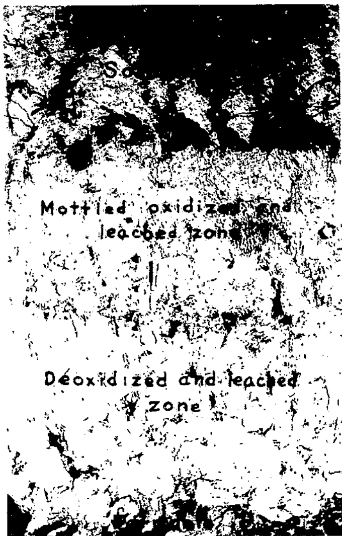
FIGURE 34.—Weathering zones in post-Farmdale Wisconsin loess.
