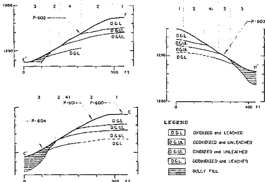
FIGURE 84.—Location of soils sampled with reference to the zonation of the Tazewell loess. P-603 and P-601 are Monona soils P-602 is a Dow soil; and P-600 a Marshall. Numbers 1, 2, 3, 4, and 41 refer to soil mapping units (table 39).
