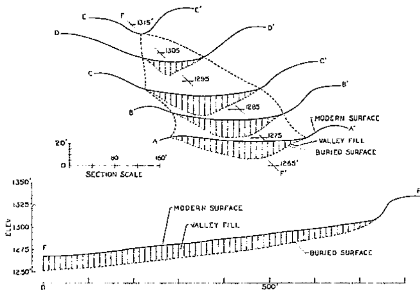
FIGURE 62.—Alluvial fill in side-valley waterway. (See fig. 61).
