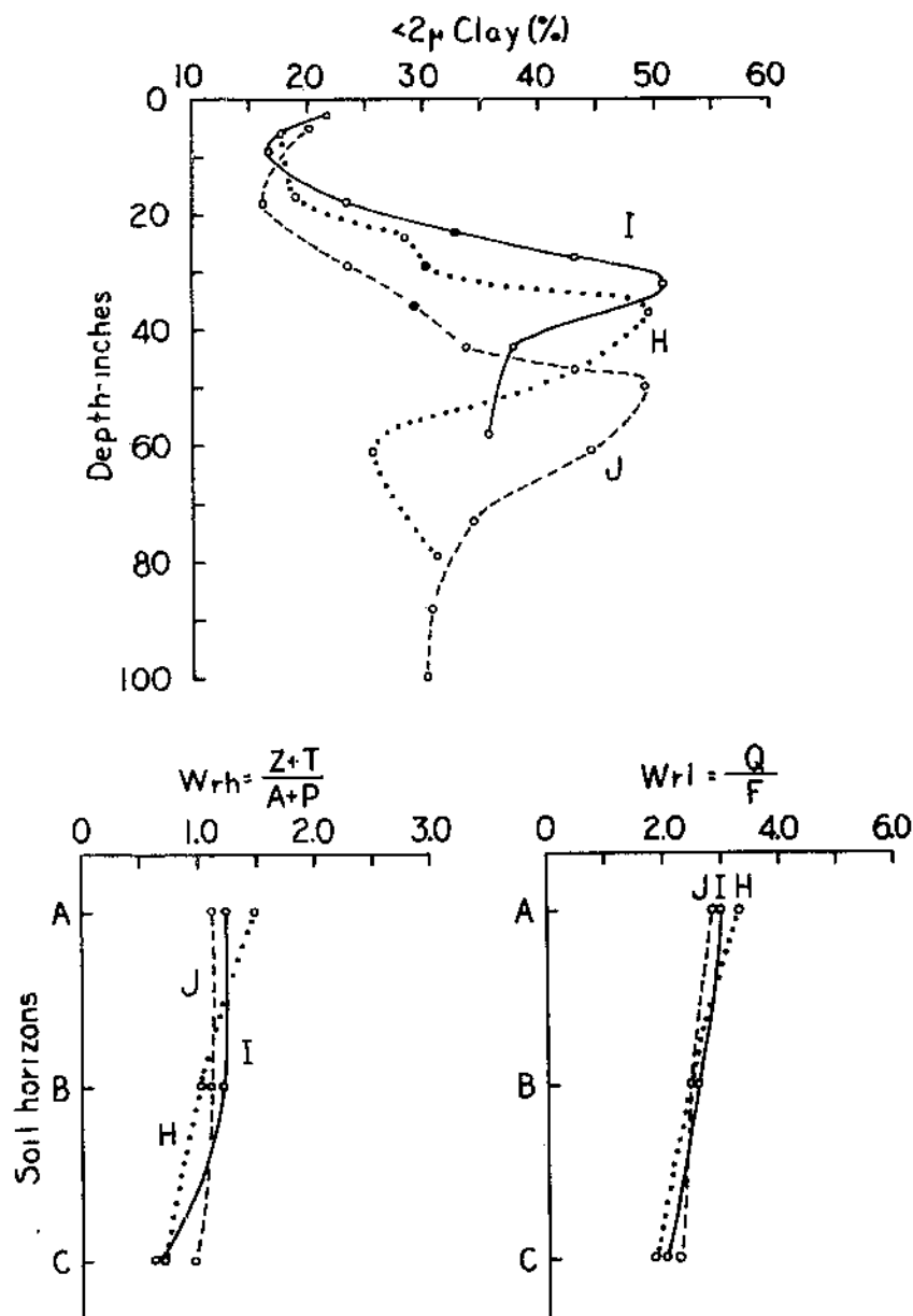
FIGURE 44.—Clay content and weathering ratios of heavy mineral fraction ( Wr_h ) and light mineral fraction ( Wr_l ) of the paleosols on the Late Sangamon pediment.
