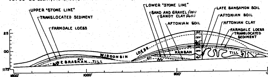
CUT 31: E 1/2 sec. 17, T76N, R39W, POTTAWATTAMIE CO.
