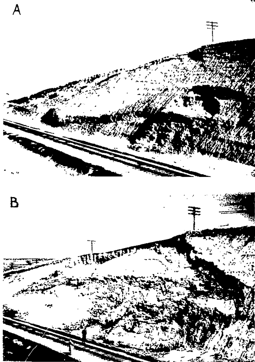
FIGURE 4.—Earthslide in cut 31, September 1953 (A) and April 1954 (B).
