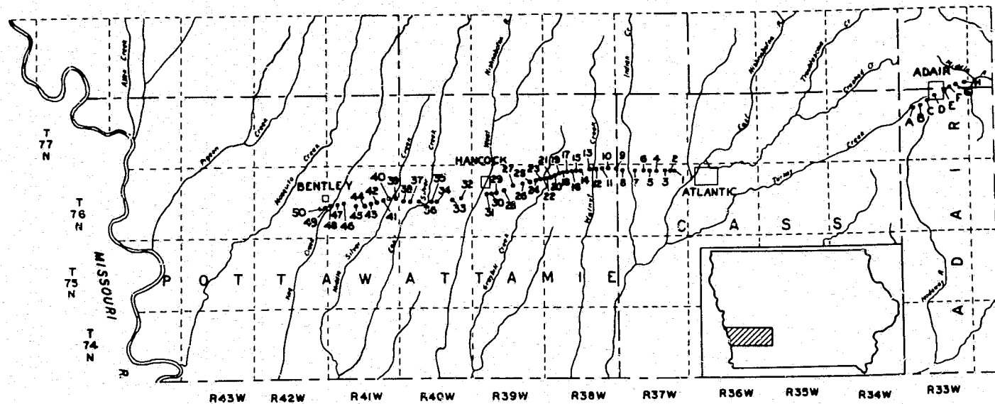
FIGURE 1.—Location of traverse in Pottawattamie, Cass, and Adair Counties, southwestern Iowa. Cuts and sections are numbered 1 to 50 and lettered A to H. (See pl. I).
