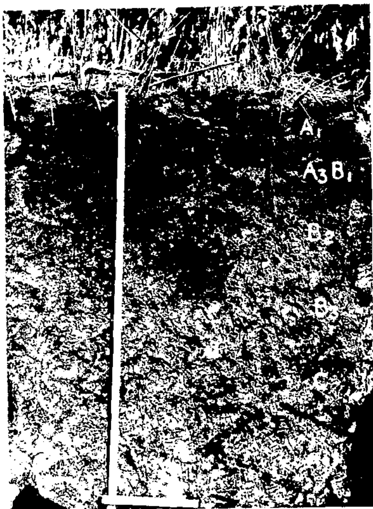
FIGURE 56.—Brunizem, Shelby loam, of Late Wisconsin-Recent age developed in Kansan till on Early Wisconsin pediment.
