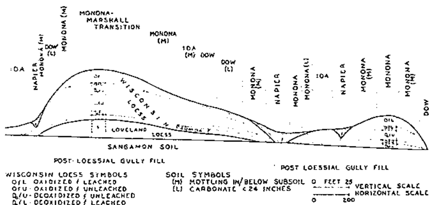
FIGURE 30.—Relationships of soils and Pleistocene stratigraphy, cut 42.
