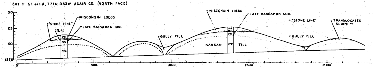
FIGURE 25.—Occurrence of Iowan and Tazewell loess on slopes that bevel the Late Sangamon pediments, cuts A, B, C, and H.
