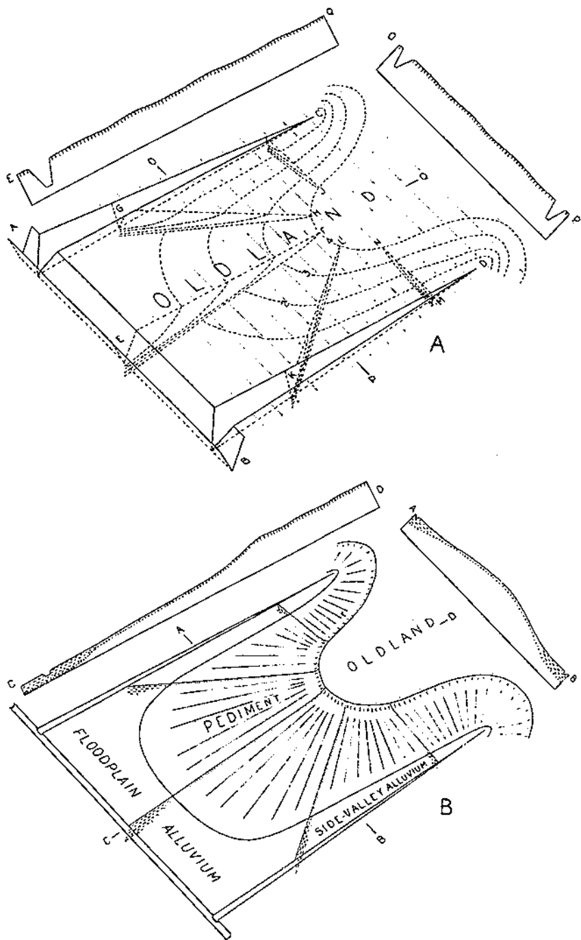
FIGURE 51.—Evolution (diagrammatically) of Late Sangamon pediment, valley-slope fan, and flood plain.
