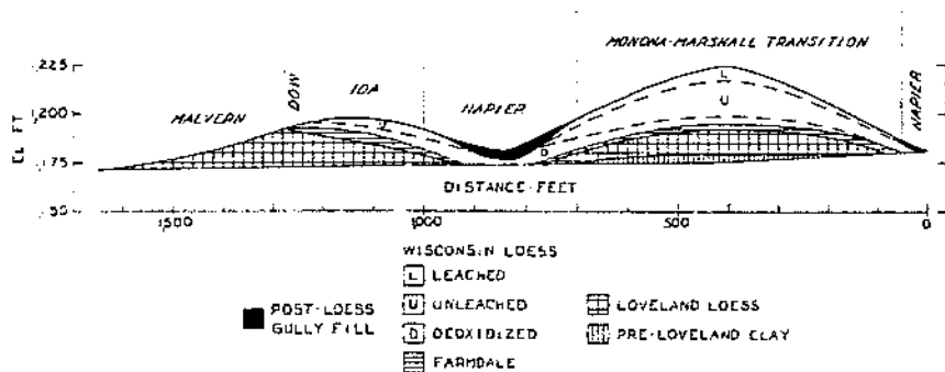
FIGURE 29.—Relationship of soils and Pleistocene stratigraphy, cut 36.
