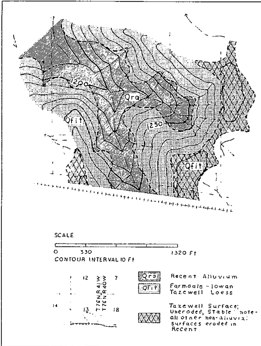
FIGURE 82.—Distribution of the Tazewell and Recent surfaces.
