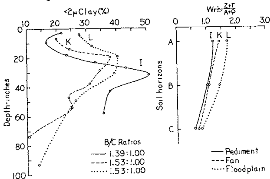
FIGURE 50.—Clay content and weathering ratios of heavy mineral fractions (Wrh) of paleosols of Late Sangamon pediment, valley-slope fan, and flood plain.
