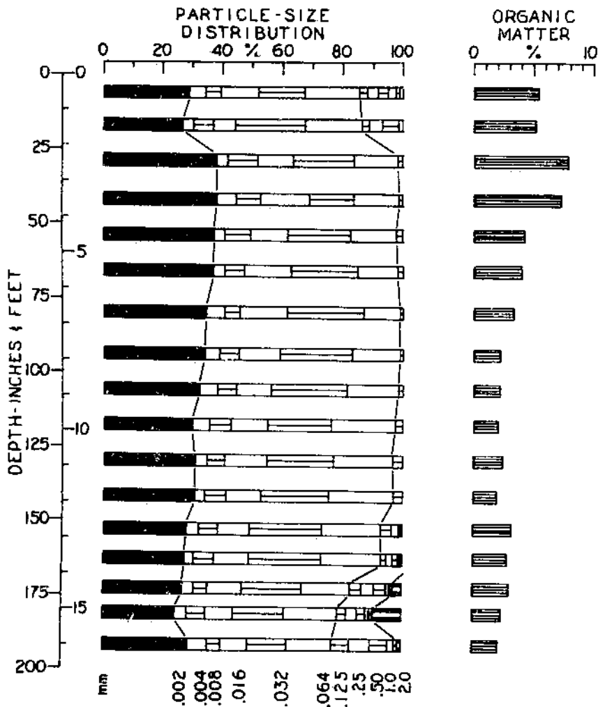
FIGURE 63.—Characteristics of the alluvium in a side-valley waterway.
