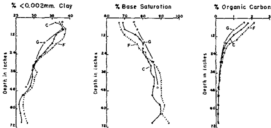
FIGURE 72.—Distribution with depth of clay ( 0.002\text{ mm.} ), percent base saturation, and organic carbon of soils in post-Farmdale loess under the late Wisconsin-Recent surface. Note: Unit 11 soils, C and G; unit 13 soil, F.
