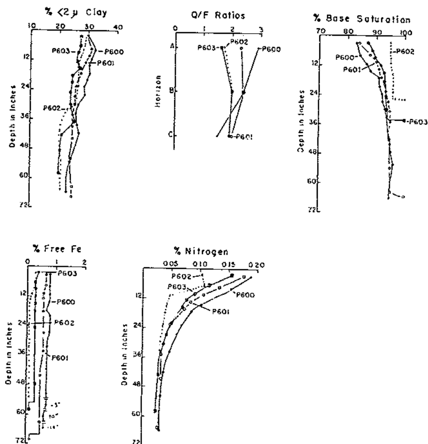
FIGURE 85.—Distribution with depth of clay ( < 2\mu ), quartz/feldspar ratios, percent base saturation, free iron, and nitrogen of soils in Tazewell loess. P-600, Marshall; P-601 and P-603, Monona; P-602, Dow.
