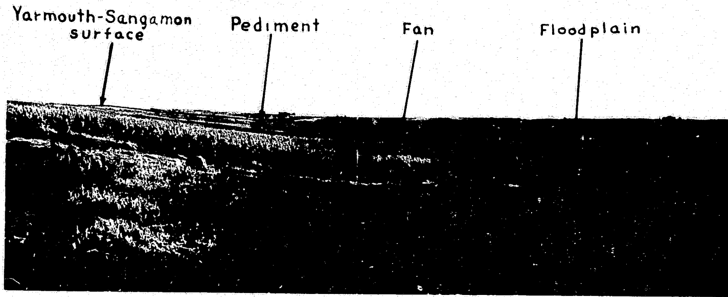
FIGURE 46.—Topographic expressions of Yarmouth-Sangamon surface and Late Sangamon pediment, valley-slope fan, and flood plain with associated valley fill in present landscape along North Turkey Creek.
