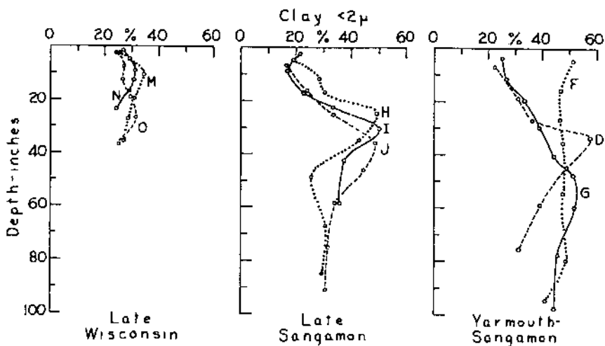
FIGURE 57.—Clay content of soils of Late Wisconsin-Recent age or Early Wisconsin pediment in comparison to paleosols of Late Sangamon and Yarmouth-Sangamon surfaces.
