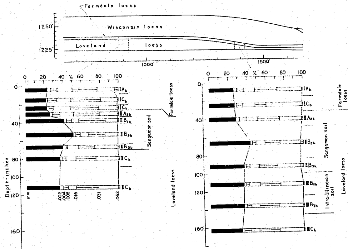
FIGURE 10.—Textures of buried soils in Loveland loess, cut 33.
