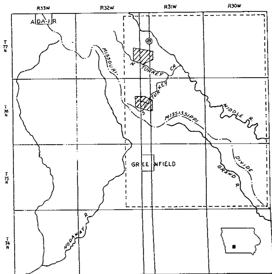
FIGURE 31.—Location of Greenfield quadrangle (bordered by broken line) and North and South Turkey Creek areas (shaded) in Adair County, Iowa.
