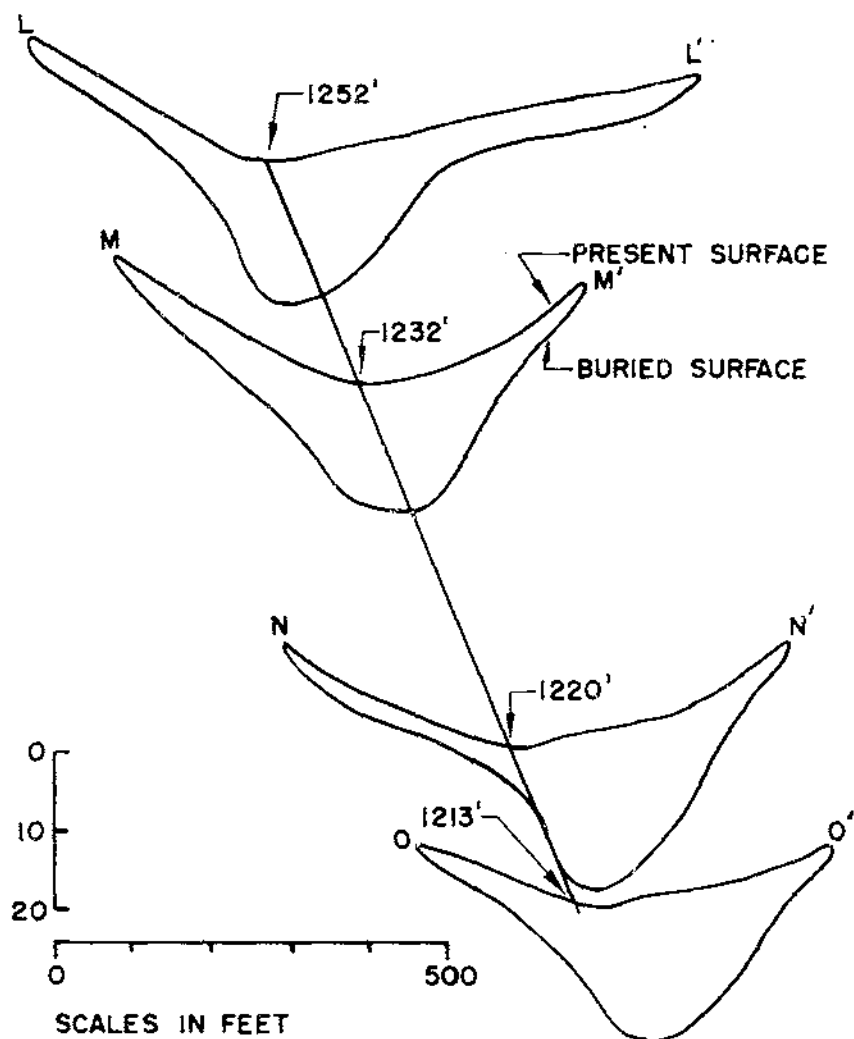
FIGURE 81.—Cross sections of the alluvial fill.
