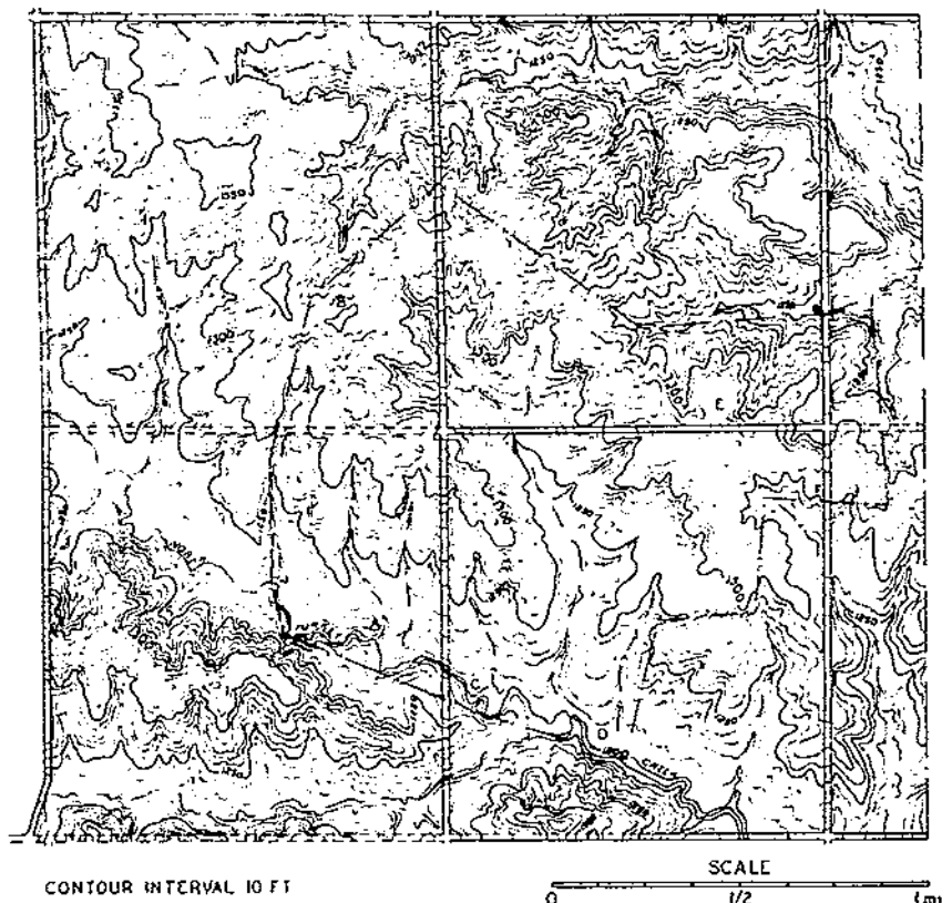
FIGURE 45.—Topographic map of North Turkey Creek area. A-B . . . F-G locate geomorphic profile sections (figs. 47, 48, 49).
