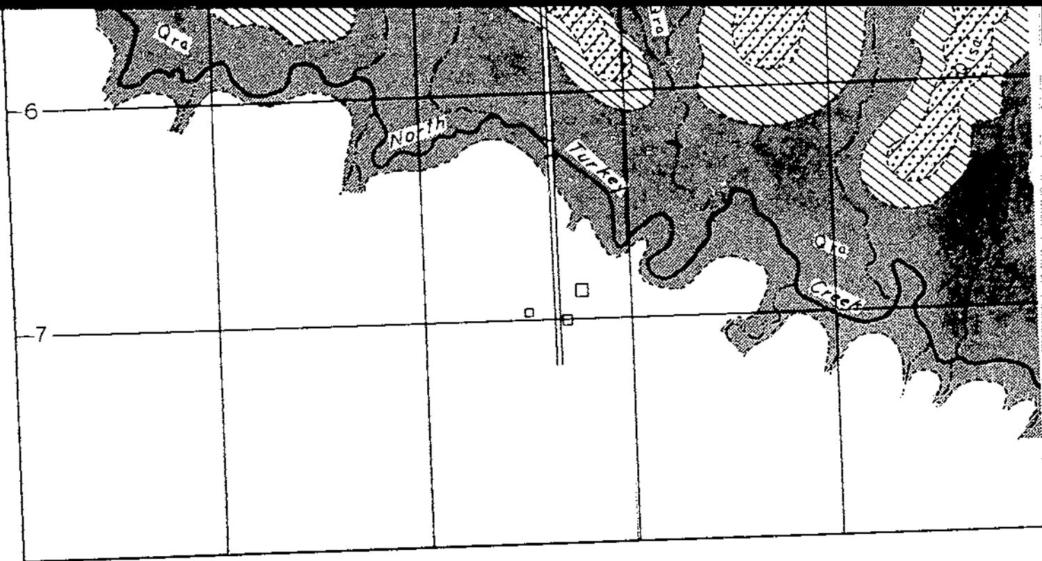
Plate IV. Geomorphic surfaces, North Turkey Creek area.
