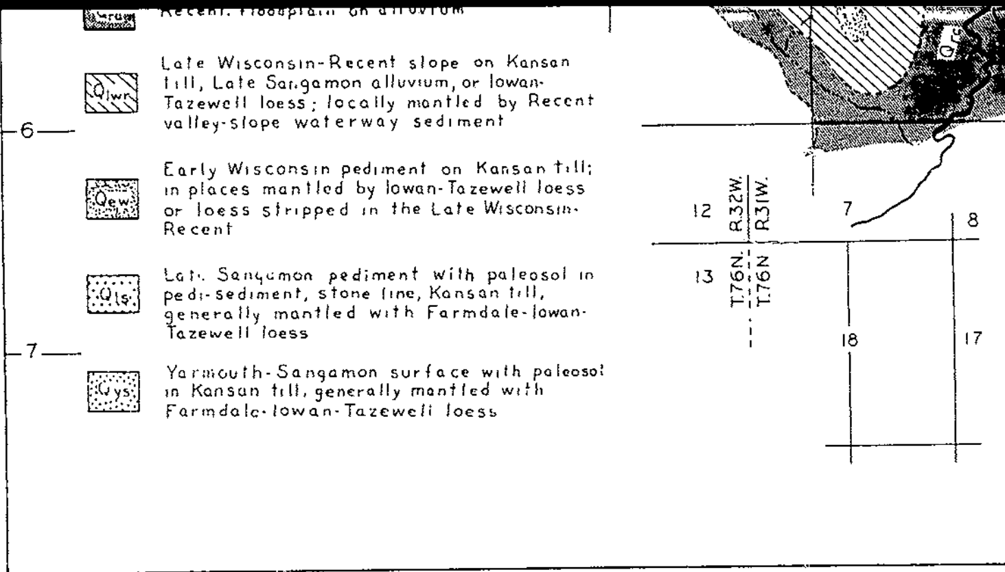
Plate II. Geomorphic surfaces, South Turkey Creek area.
