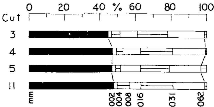
FIGURE 7.—Textures of Yarmouth lake clay, cuts 3, 4, 5, and 11.
