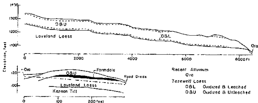
Figure 3.—Distribution of sediments along and across the long axes of ridge crests in Magnolia watershed.
