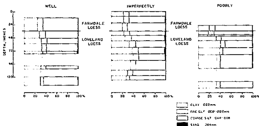
Figure 18.—Particle-size distribution in well, imperfectly, and poorly drained Sangamon paleosols.
