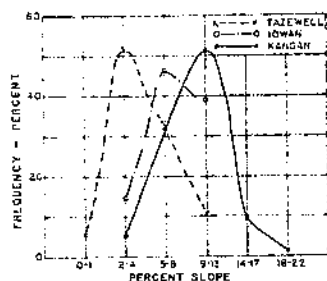
Figure 7.—Frequency curves of slopes on the ground surface exclusive of alluvial areas in the Kansan, Iowan, and Tazewell drift areas in Sac County and Crawford County, Iowa.
