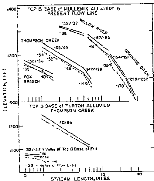
Figure 40.— k values of the base of the Mullenix and Turton fills and of the present stream channels in the Willow River and Thompson Creek valleys. Only a few of the points used in computing the k values are shown.
