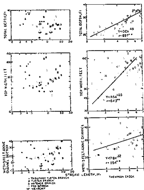
Figure 31.—Properties of entrenched streams in Thompson Creek watershed. (**Significant at 1-percent level, *significant at 5-percent level.)
