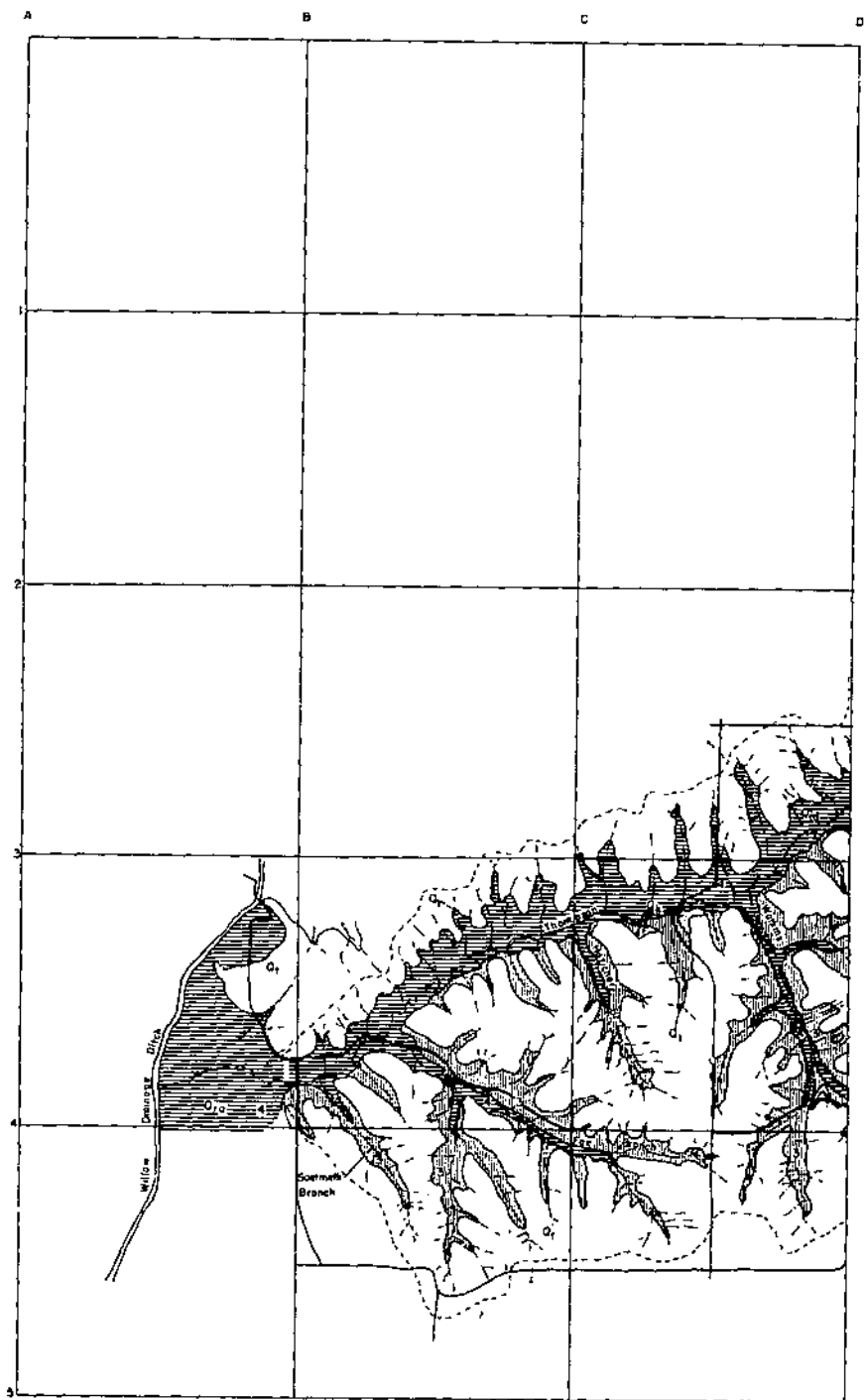
Plate 1.—Surficial deposits of
