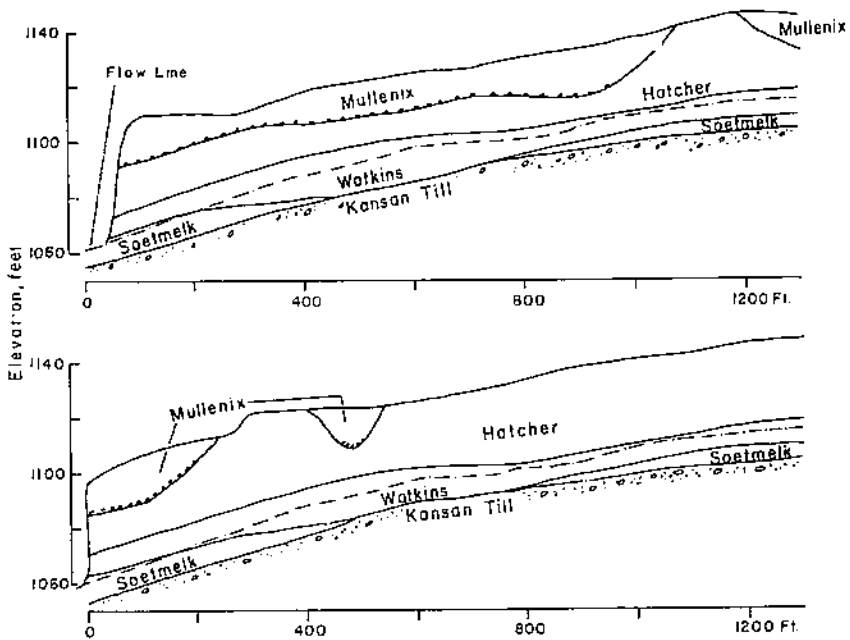
Figure 10.—Relation between the Hatcher and Mullenix fills in the lower part of Soetmelk Branch, Thompson Creek watershed.
