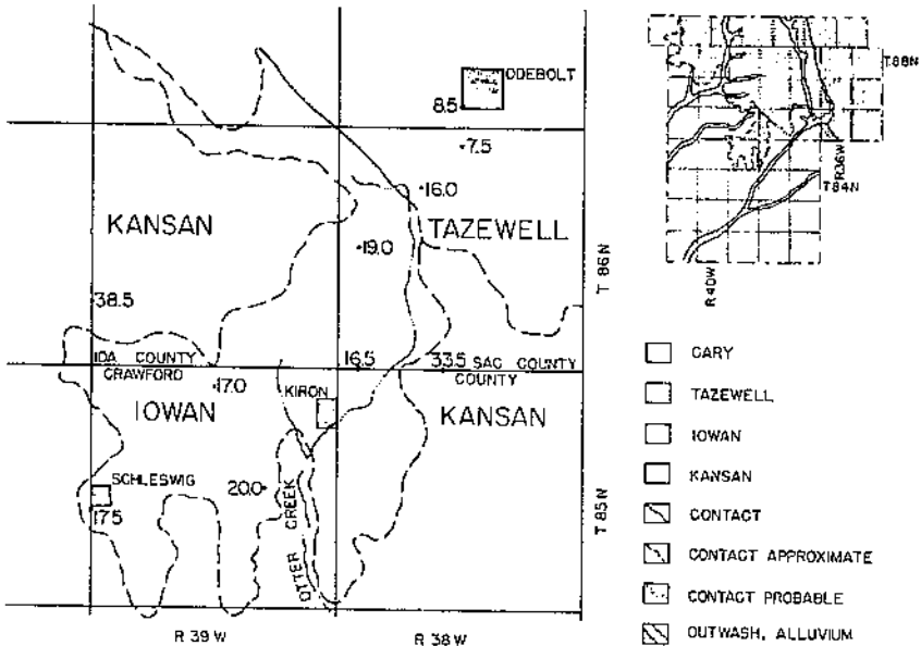
Figure 6.—Left, areal distribution of Iowan drift in north-central Crawford County, southeastern Ida County, and southwestern Sac County, Iowa. (Numbers beside dots give loess thickness in feet.) Right, distribution of Cary, Tazewell, and Iowan drift areas north of T. 87 N., R. 40 W. (after Ruhe 1950).
