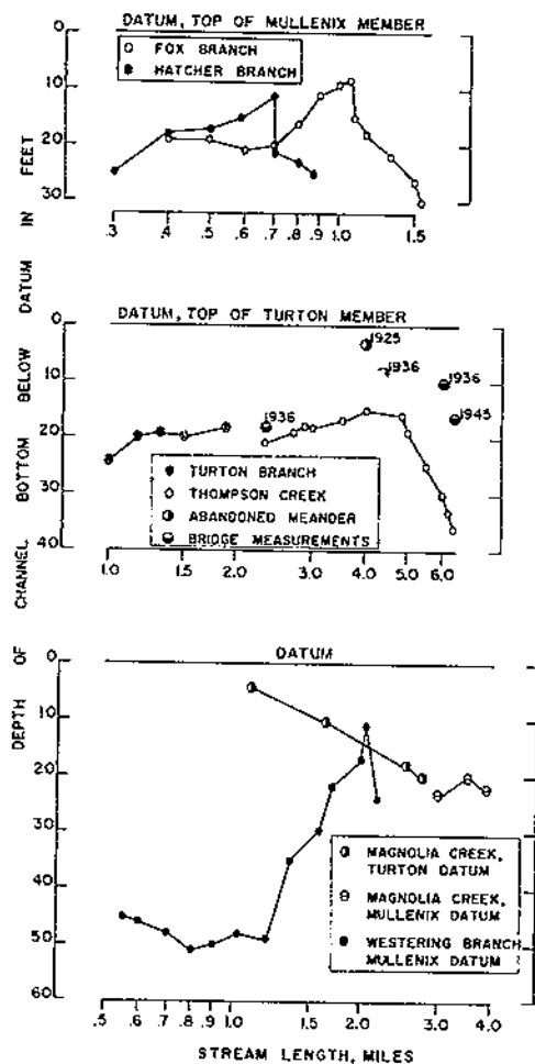
Figure 32.—Depth of modern erosion of selected streams in Thompson and Magnolia watersheds.
