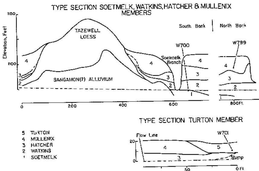
Figure 9.—Sequence of sediments at type sections of the De Forest formation; W700, W701, and W799 are radiocarbon samples.
