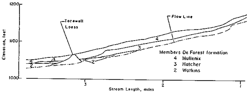
Figure 13.—Members of the De Forest formation exposed in trench of Magnolia Creek.
