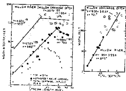
Figure 24.—Relation of top width, width 5 feet above channel bottom, and depth of channel bottom below flood plain to stream length and of top width to depth in Willow River and drainage ditch. Willow River is upstream from the head of the drainage ditch 2\frac{1}{2} miles north of the Monona-Harrison county line. (**Significant at 1-percent level, *significant at 5-percent level.)
