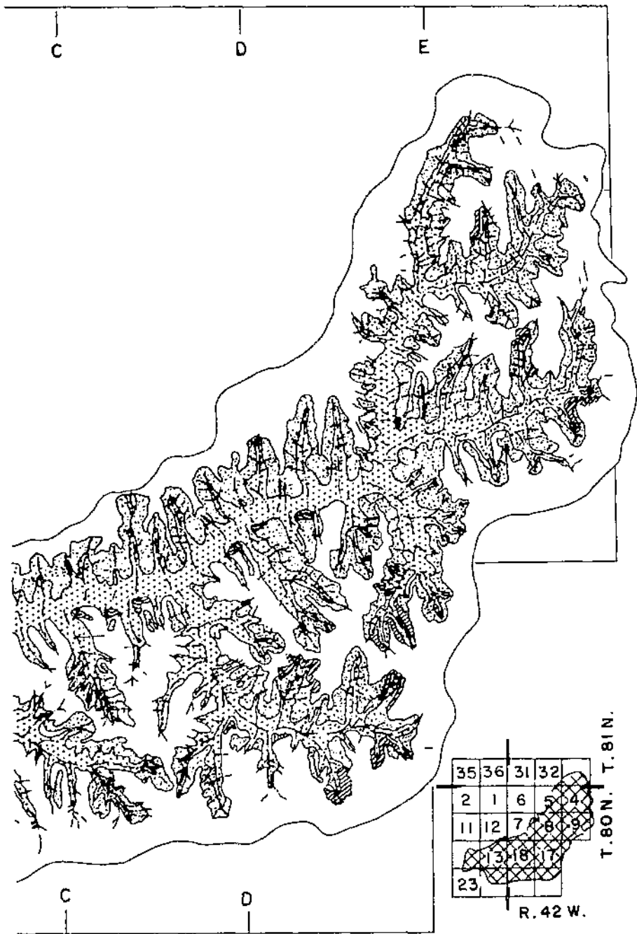
Thompson Creek watershed.
