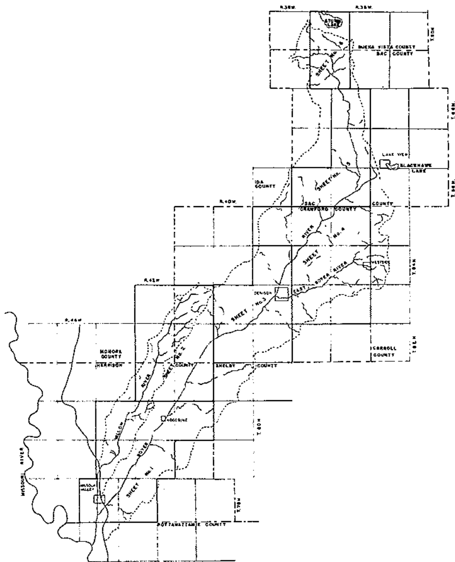
Plate 3.—Distribution of late Sangamon, Tazewell, and Cary terraces in the Boyer and Willow valleys (index).
