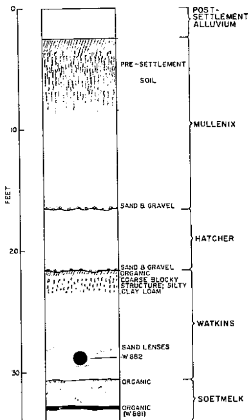
Figure 17.—Members of the De Forest formation exposed in the west bank of Willow drainage ditch in SW \frac{1}{4} sec 11, T. 80 N., R. 43 W., Harrison County, Iowa. The section is 100 feet north of an unnamed tributary that enters from the west. W881 and W882 are radiocarbon samples.
