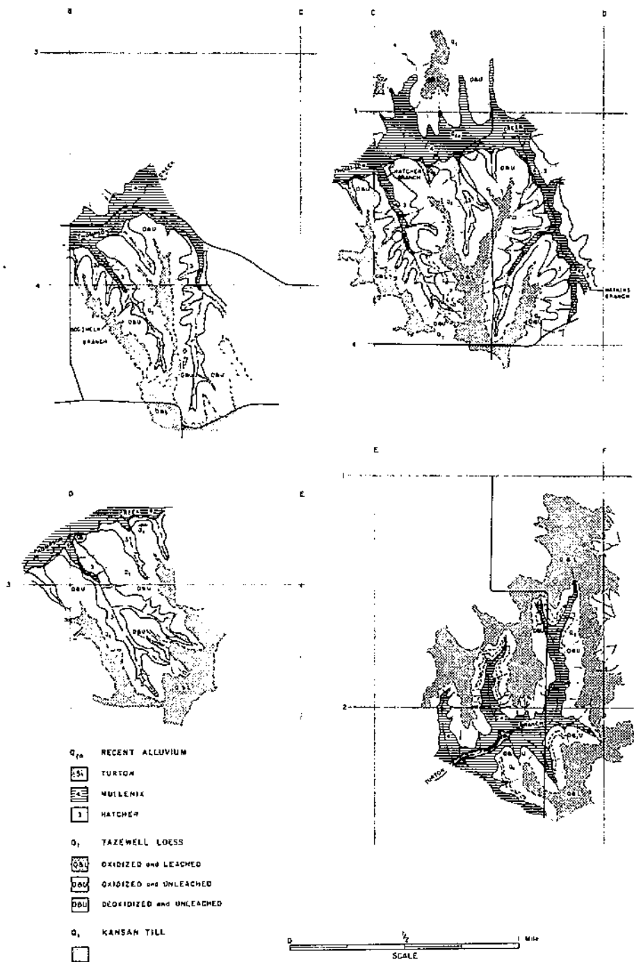
Plate 4.—Surfacial deposits and areal distribution of weathering zones of Tazewell loess in selected areas of Thompson Creek watershed.
