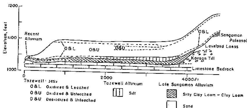
Figure 5.—Relation of late Sangamon terrace deposits to upland deposits at the Logan quarries.
