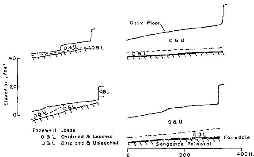
Figure 38. Relation between buried geomorphic surfaces and floor of valley-slope gullies.
