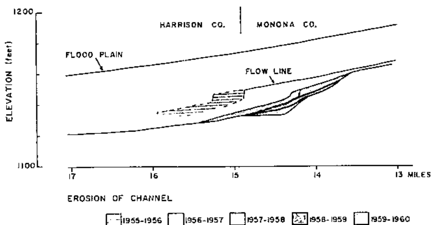
Figure 28.—Changes in the Willow drainage ditch since 1955.
