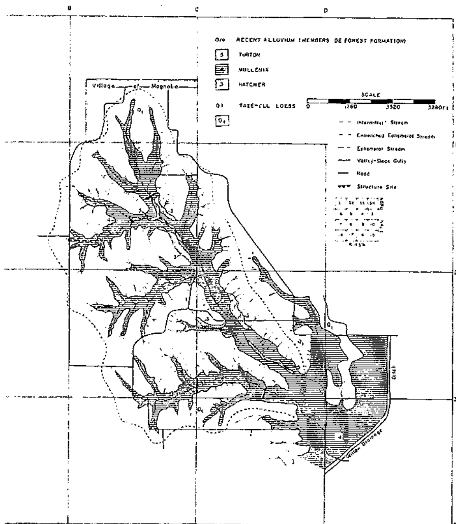
Plate 2.—Surficial deposits of Magnolia watershed.
