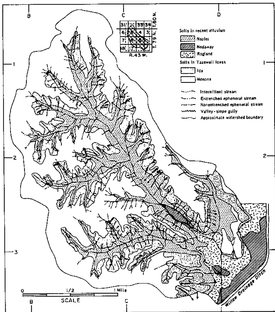
Plate 7.—Soils in Magnolia watershed (G. H. Simonson).
