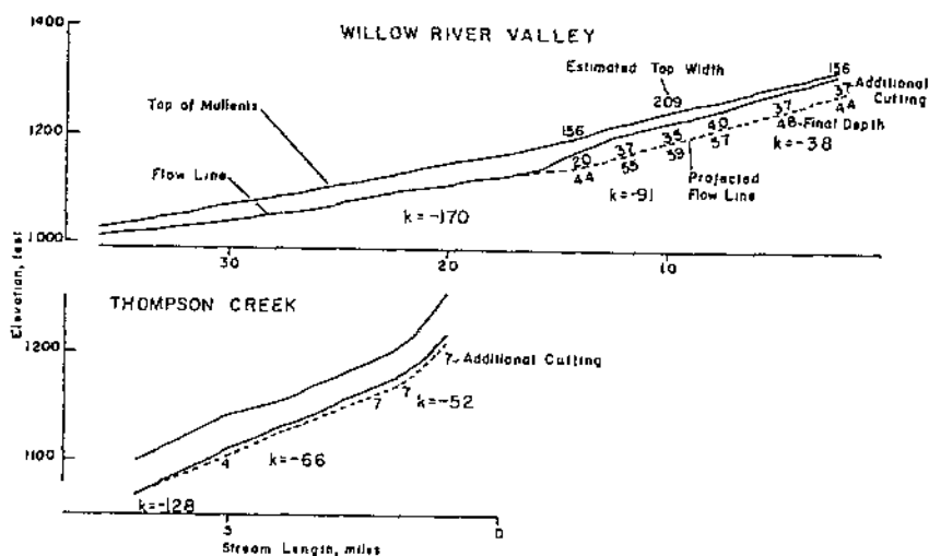
Figure 41.—Predicted profiles of the Willow River and drainage ditch and Thompson Creek (estimated by projecting k values upstream).
