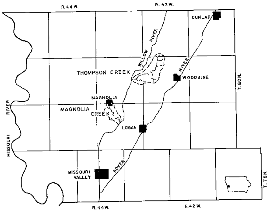
Figure 1.—Location of Thompson Creek and Magnolia watersheds, Harrison County, Iowa.
