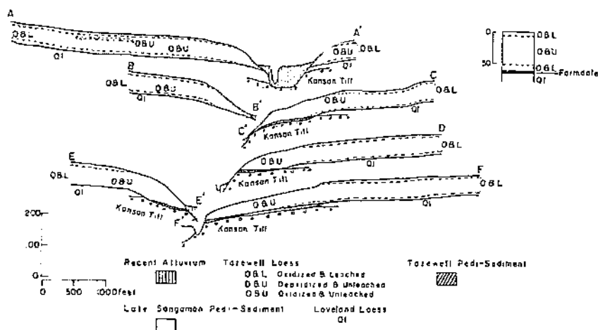
Figure 2.—Distribution of sediments along the long axes of ridge crests in Thompson Creek watershed. The relation of the Farmdale to other sediments is shown in the upper right corner.
