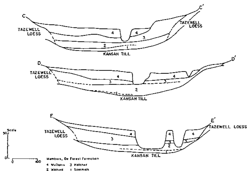
Figure 14.—Distribution of members of the De Forest formation across the long axis of Thompson Creek valley—C-C', D.43, 2.57-D.48, 2.69; D-D', C.59, 3.05-C.57, 3.19; E-E', B.22, 3.59-B.28, 3.74 (pl. 1).
