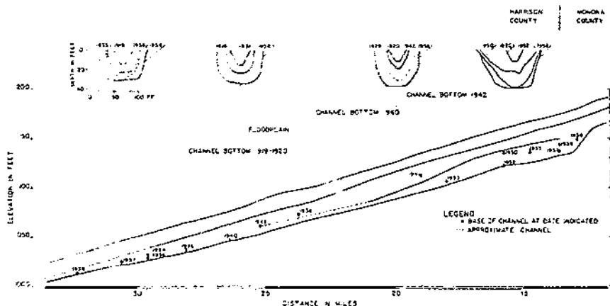
Figure 25.—Profile of Willow drainage ditch in Willow River valley and post-construction changes.
