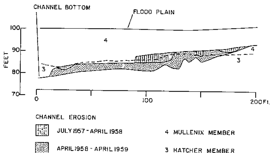
Figure 33.—Changes in the channel of Fox Branch at the site of a nickpoint.
