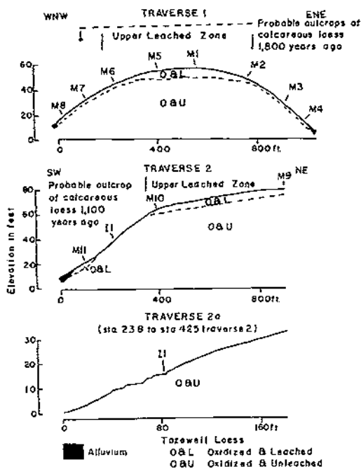
Figure 20.—Relation of Monona and Ida soils to the weathering zones of Tozwell loess.
