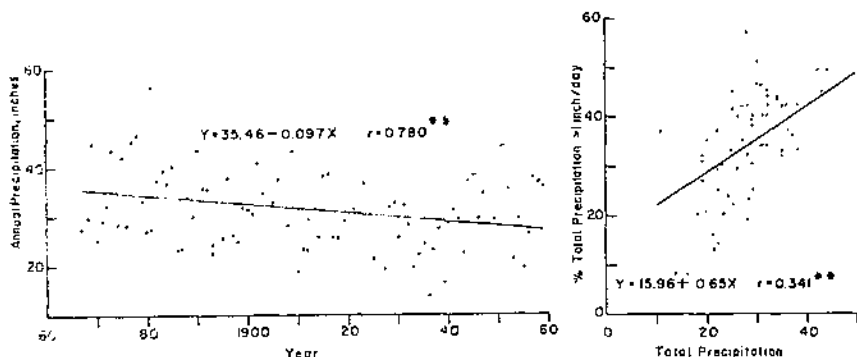
Figure 34.—Annual precipitation at Logan, Iowa, from 1867 to 1959 and percentage of annual precipitation from storms of 1 inch or more per day.
