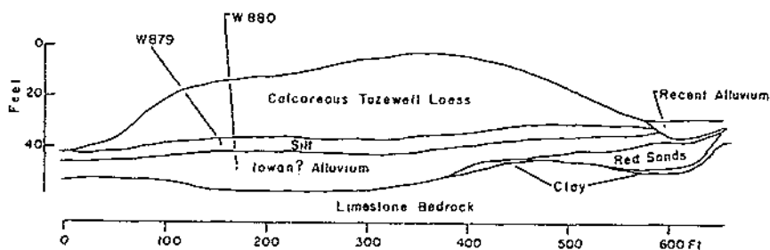
Figure 8.—Sediments exposed in the north face of a quarry at Logan, sec. 20, T. 79 N., R. 42 W., Harrison County, Iowa.
