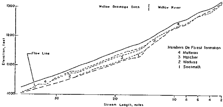
Figure 12.—Members of the De Forest formation exposed in trenches of Willow drainage ditch and Willow River.
