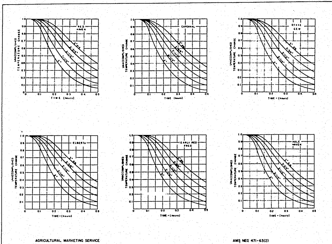
FIGURE 4.—Cooling characteristics of six peach varieties, based on experimentally determined values of "effective" thermal diffusivity. Temperature at center of fruit.
