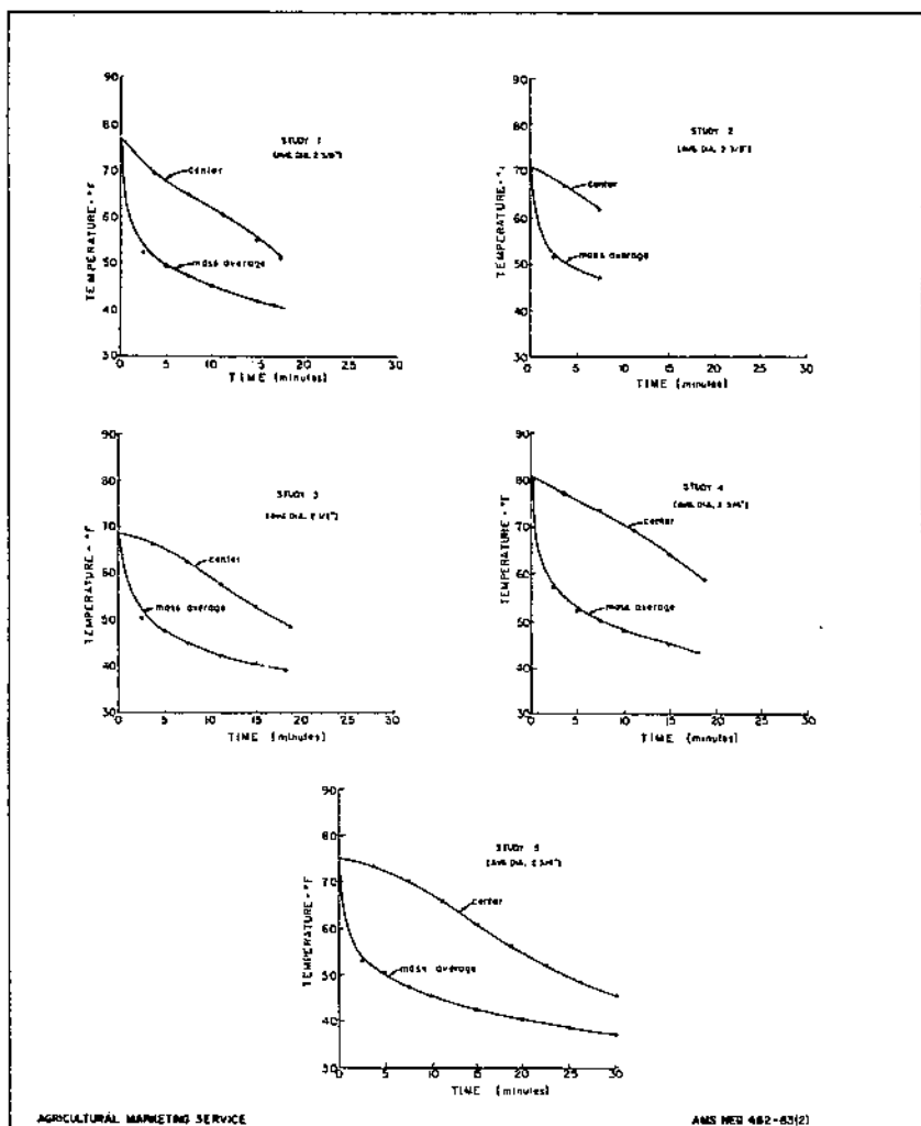
FIGURE 15.—Center and mass-average temperatures of peaches 2 \frac{3}{8} to 2 \frac{3}{4} inches in diameter, in the middle of container during typical cooling in conventional flood-type hydrocoolers.
