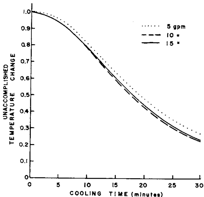
FIGURE 10.—Effect of water flow rate on cooling 2½-inch Elberta peaches, using spray nozzles for fine spray. Temperature measured at the center of fruit located on the bottom of ¾-bushel baskets.
