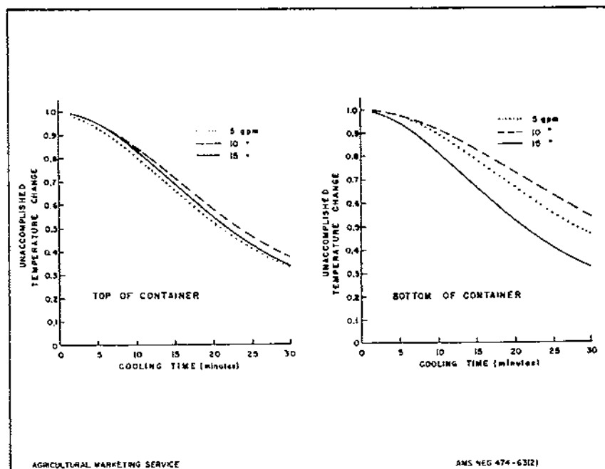
FIGURE 9.—Effect of water flow rate on cooling 3-inch-diameter Hale Haven peaches using shower nozzles for coarse spray. Temperatures measured at the center of fruit located at the top and bottom of \frac{1}{4} -bushel baskets.
