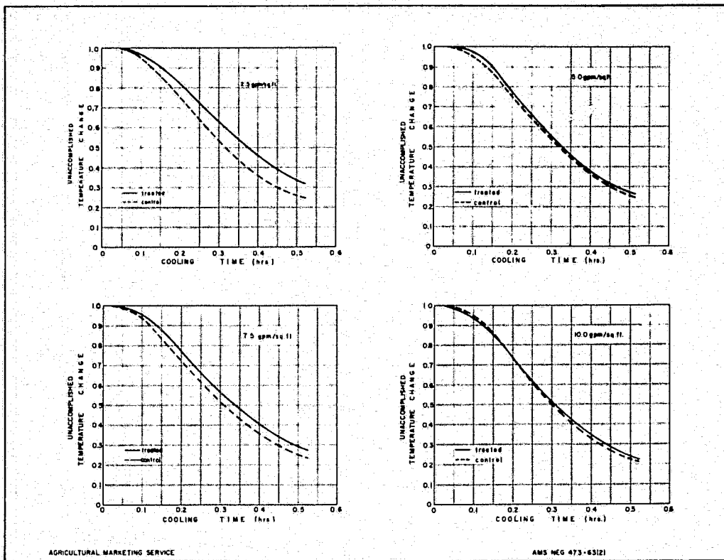
FIGURE 8.—A comparison of the effect of a wetting agent (treated) to no wetting agent (control) in the cooling water at specified flow rates on 2¼-inch-diameter Elberta peaches. Temperature measured at center.
