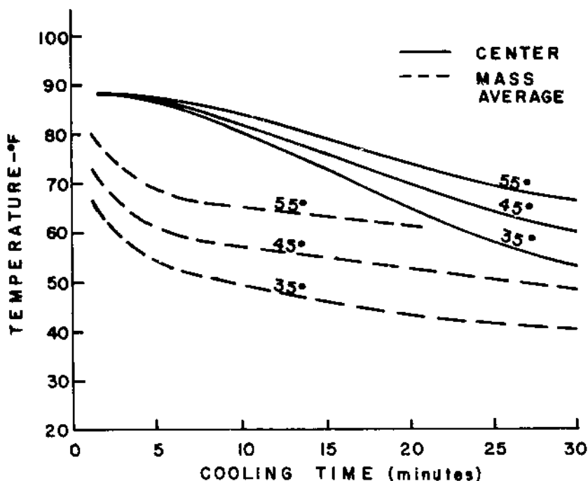
FIGURE 11.—Effect of water temperature on cooling 3-inch-diameter Hale Haven peaches. Center and mass-average temperatures. Average of top, middle, and bottom of \frac{3}{4} -bushel baskets.
