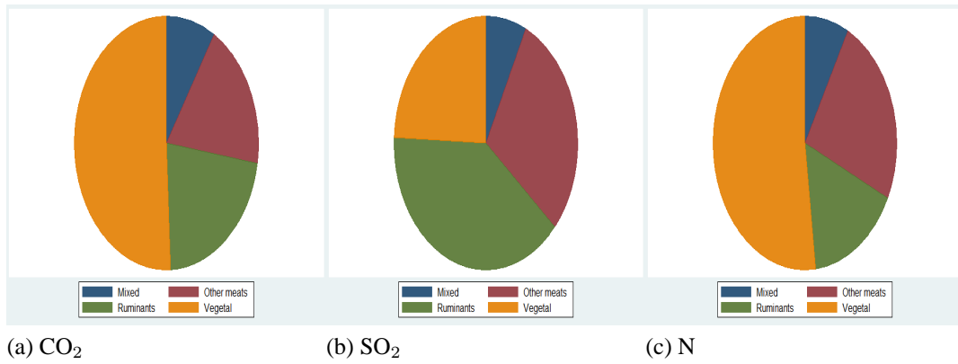
Figure 1: Contribution of Aggregated Food Groups to CO 2 , SO 2 and Nitrates Emissions
