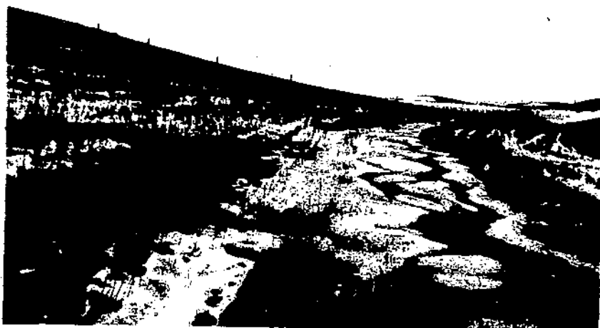
FIGURE 24.—Snow and ice in the channel of terrace 6, December 26, 1932.
