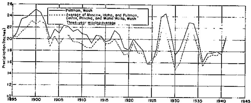
FIGURE 4.—Precipitation at different locations in the problem area for the period 1893-1941.
