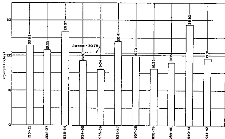
FIGURE 12.—Annual and average precipitation for the 11-year period July 1, 1931, to June 30, 1942, from field 3 gage at the Soil Conservation Experiment Station, Pullman, Wash.
