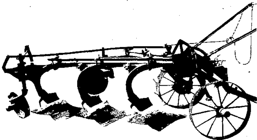
FIGURE 22.—Three-bottom, 16-inch plow rebuilt to give 26-inch clearance below beam and equipped with experimental moldboards 6 inches wide.
