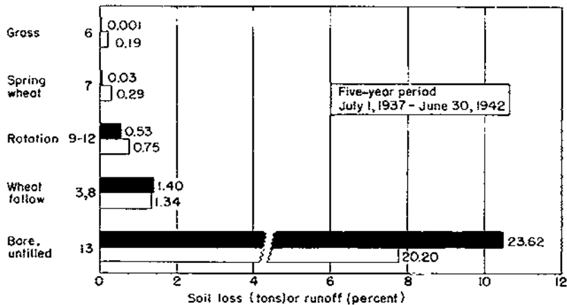
FIGURE 17.—Effect of cropping system on soil and water losses. Average annual values for the south control plots.
