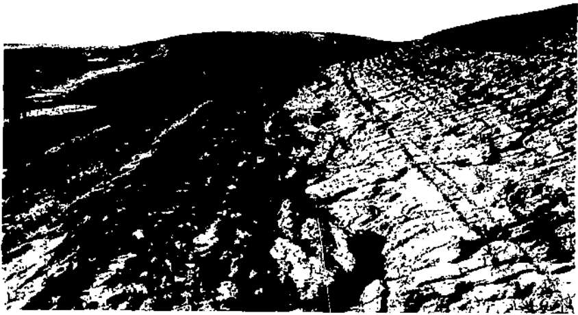
FIGURE 25.- Washing in the channel of terrace 15, fall of 24 inches per 100 feet, April 15, 1932.
