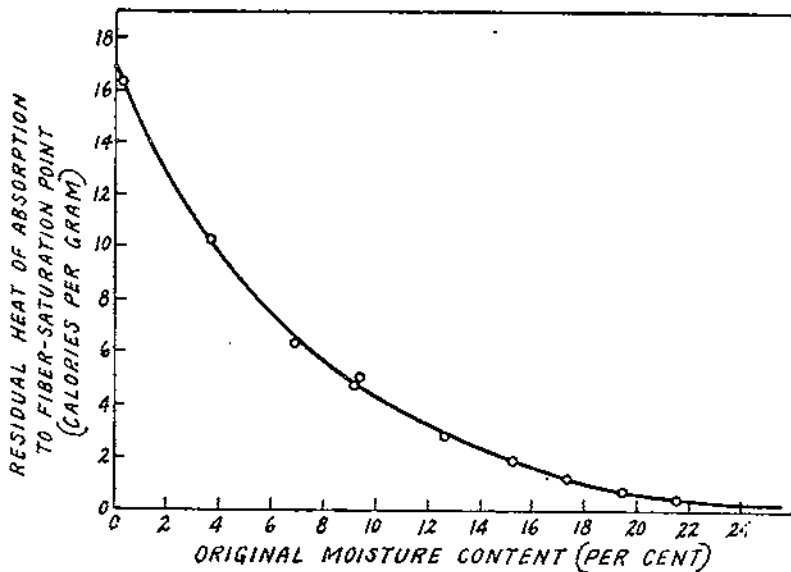
FIGURE 3.—The relation between change in original moisture content and residual heat of absorption for pine-wood flour as the moisture content increases to the fiber-saturation point
