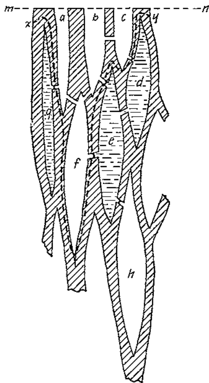
FIGURE 14.—A third stage in the drying of an idealized wood structure: a , b , c , d , e , f , g , and h , fiber cavities in an idealized wood structure; m , n , exterior surface of the piece of wood; xy , surface of the liquid in the cavities from which evaporation takes place
