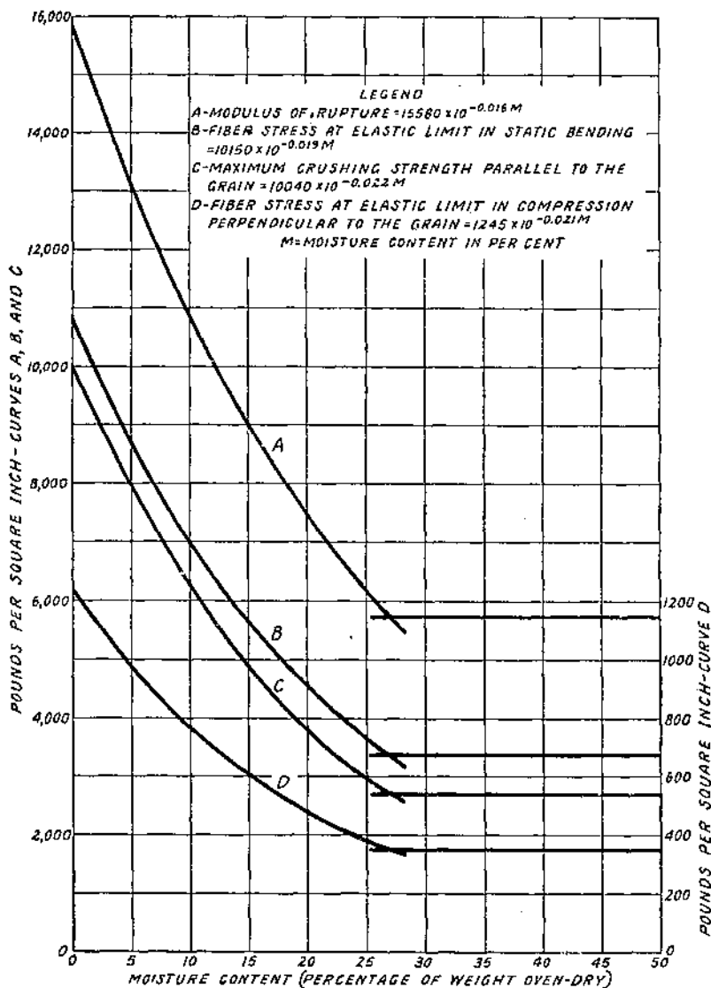
FIGURE 5.—The relation between the strength and the moisture content of small, clear specimens of Sitka spruce
