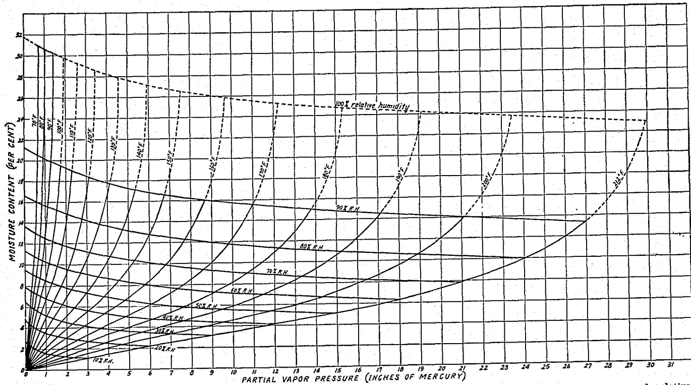
FIGURE 4.—The moisture-content values of Sitka spruce at equilibrium with various temperatures, partial vapor pressures, and relative humidities
