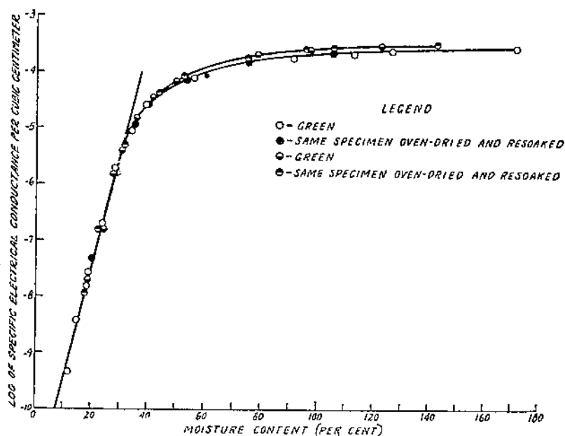
FIGURE 8.—The effect of moisture content on the specific electrical conductance of nonextracted redwood
