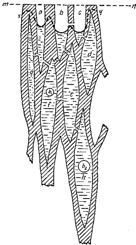
FIGURE 12.—An early stage in the drying of an idealized wood structure: a , b , c , d , e , f , g , and h , Fiber cavities in an idealized wood structure; b_1 and b_2 , bubbles of entrapped air or other gas; mn , exterior surface of the piece of wood; xy , surface of the liquid in the cavities from which evaporation takes place
