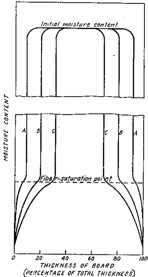
FIGURE 9.—The moisture-gradient in wood at three stages of drying when there is no movement of free water: A, at an early stage in drying; B and C, at successive later stages
