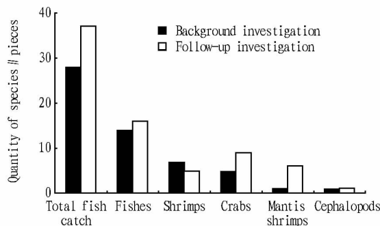
Fig. 2 Total fish catch of nekton species in reef area through trawling background investigation and follow-up investigation
