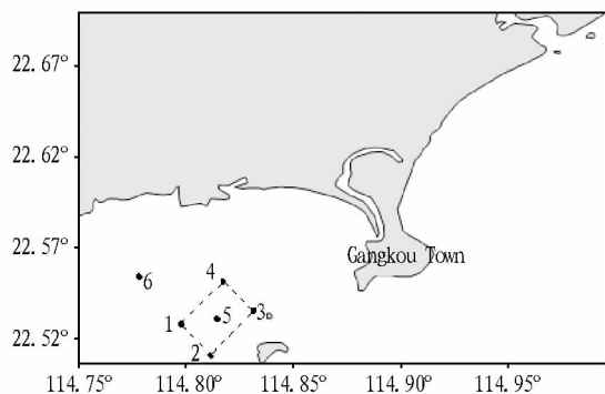
Fig. 1 Investigation station of Daxingshan artificial reef area in Huidong County
