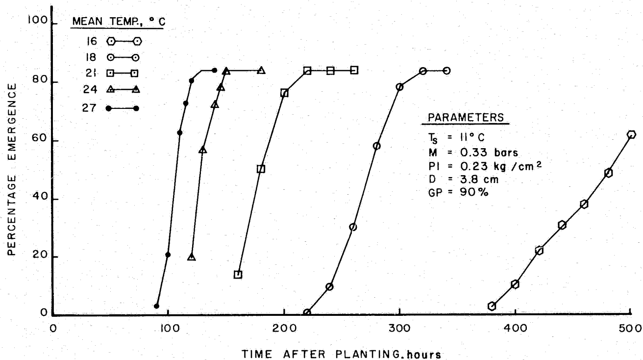
FIGURE 4.—Predicted cotton emergence from sinusoidal temperature regimes having different mean temperatures with a common daily temperature swing of 11^\circ\text{C} .
