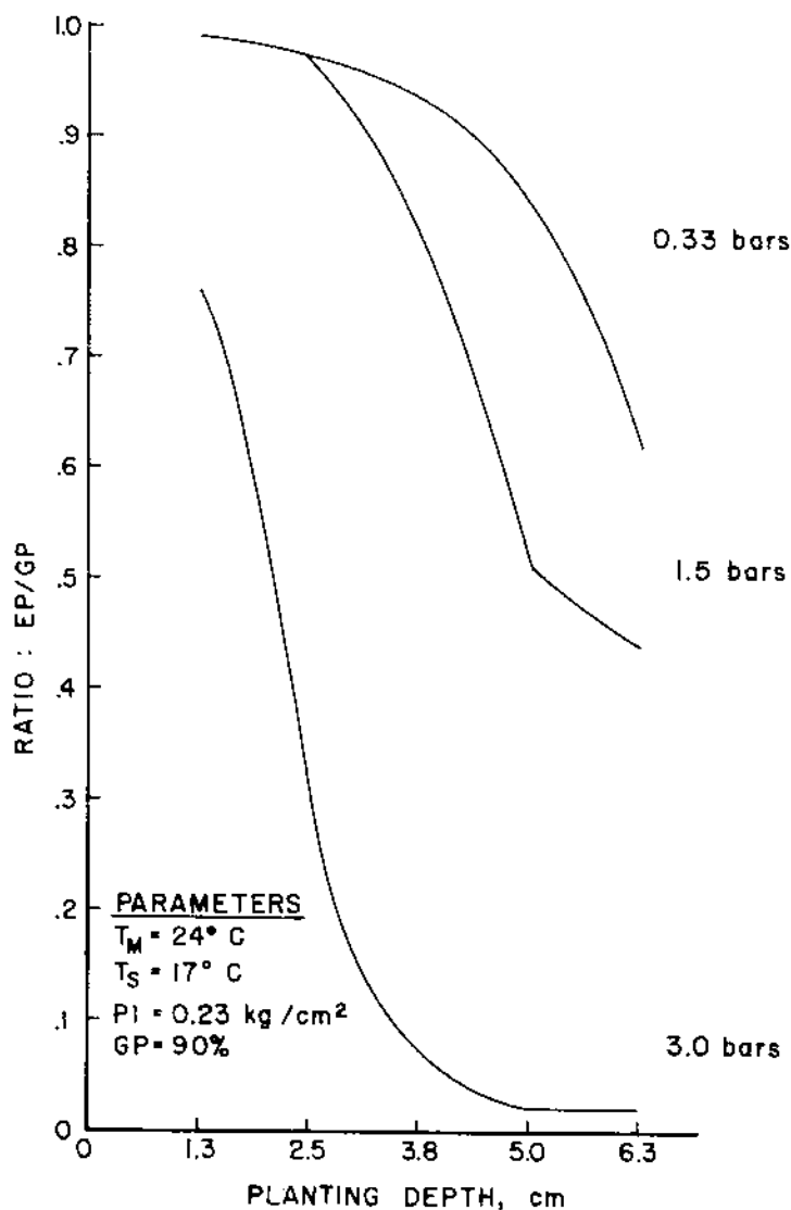
FIGURE 14.—Relationship between the ratio of maximum emergence percentage standard germination percentage and planting depth for different soil-moisture tensions.
