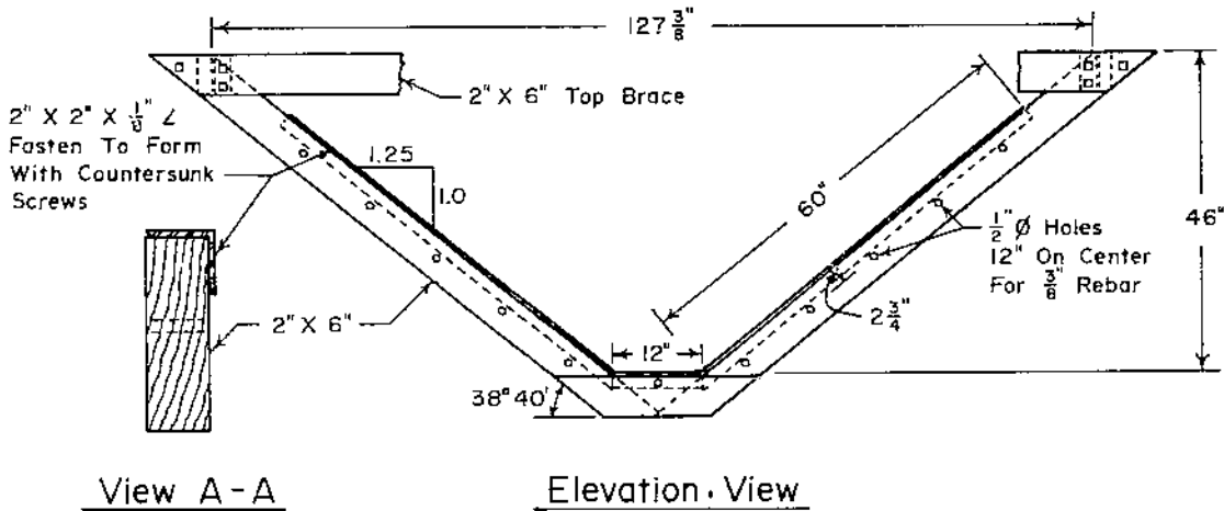
FIGURE 7.—Form for casting the throat section of a trapezoidal fume in an unlined ditch.
