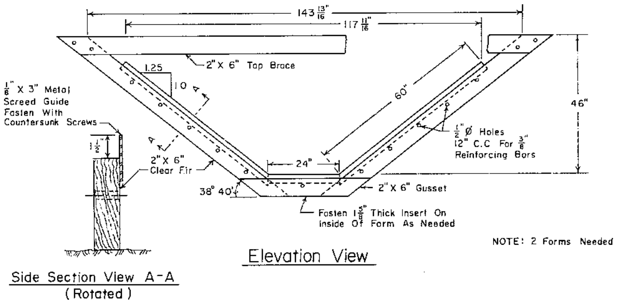
FIGURE 8.—Form for casting the end sections of a fume in an unlined ditch.
