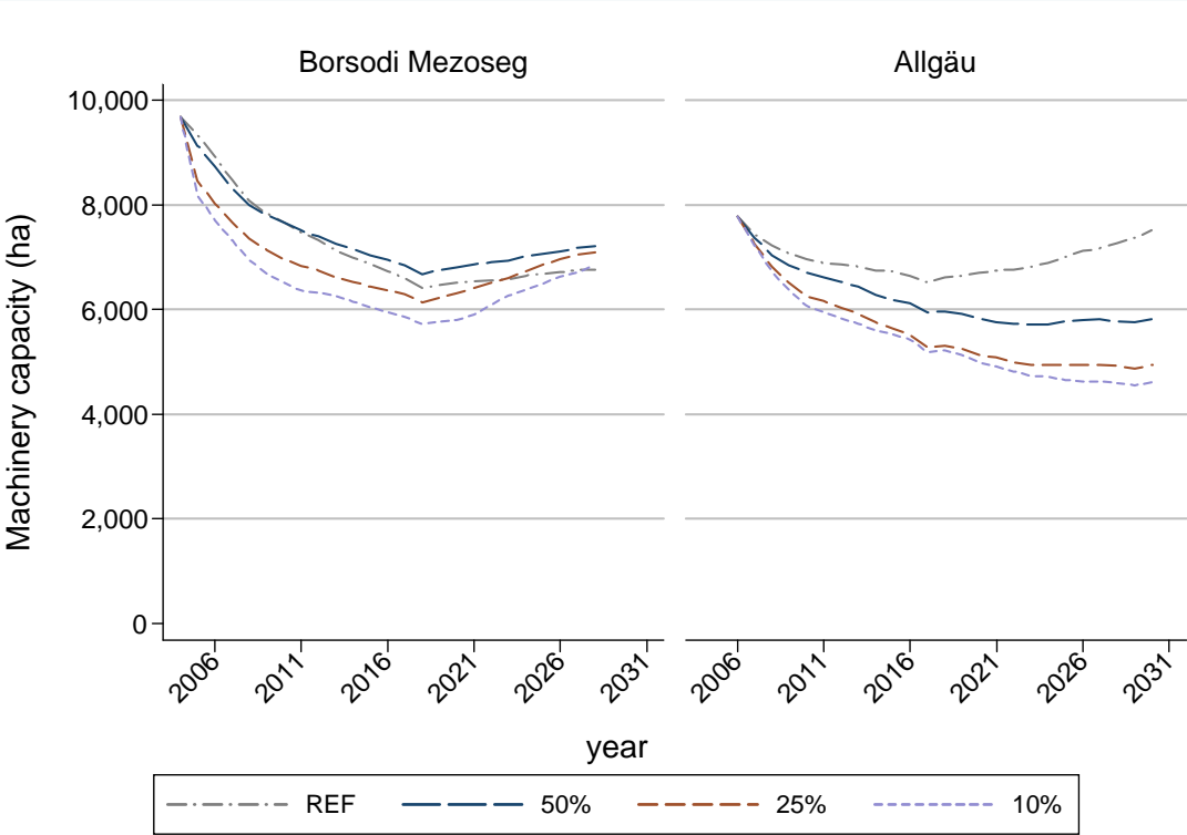
Figure 0-9 Development of machinery capacity in Borsodi Mezőse and Allgäu
