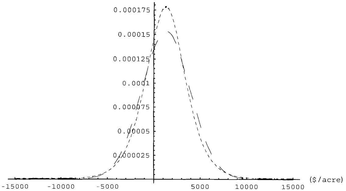
Figure 6. Fitted Normal Density — — and Fitted Restricted HT Transformation - - - - of CSA Real Net Income per Acre in the Northeastern United States
