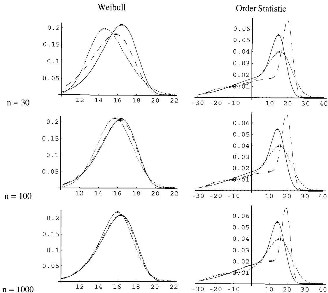
Figure 4. Population Density, g(x) ———, Fitted Population Density, \hat{g}(x) - - -, and Fitted Restricted HT Transformation, f(x) - - -, for Weibull and Order Statistic Populations by Sample Size ( n )
