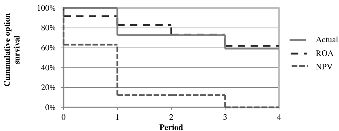
Figure 4. Survival functions of actual and optimal investment behavior according to NPV and ROA.
