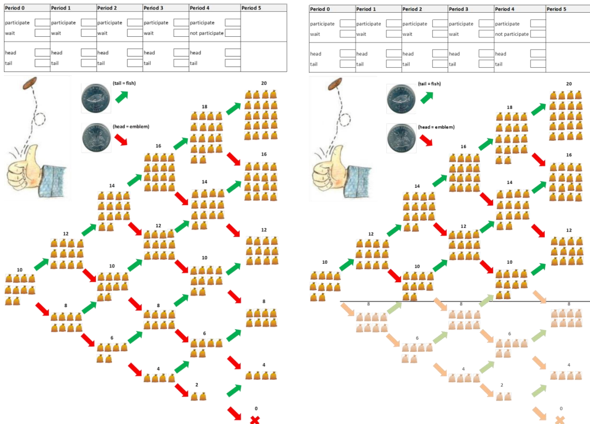
Figure 1. Graphical display of the binomial tree of potential investment returns (in thousand points) in the NPF (left) and WPF treatment (right).
