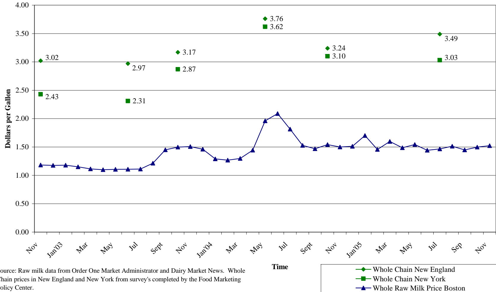
Figure 3. Weighted Average Chain Store 3.25% Whole Milk Prices in New York and New England and Repsective 3.5% Whole Raw Milk Prices
