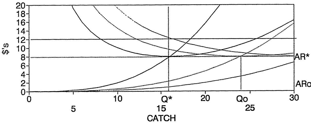
FIGURE 1: FISHING INDUSTRY COST CURVES OPEN ACCESS'; TAC ONLY"; & OPTIMAL
