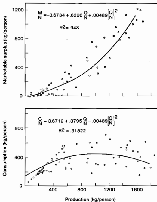
Fig. 2. Relationships between household consumption, marketable surplus, and production for Philippine rice farms (Toquero et al. 1975).
