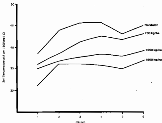
Figure 5. The effect of various amounts of mulch (dead Stylo) on soil temperatures over a 6 day period.
