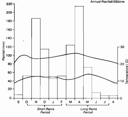
Figure 13. Mean monthly rainfalls, maximum temperatures, and minimum temperatures at Machakos, Kenya.
