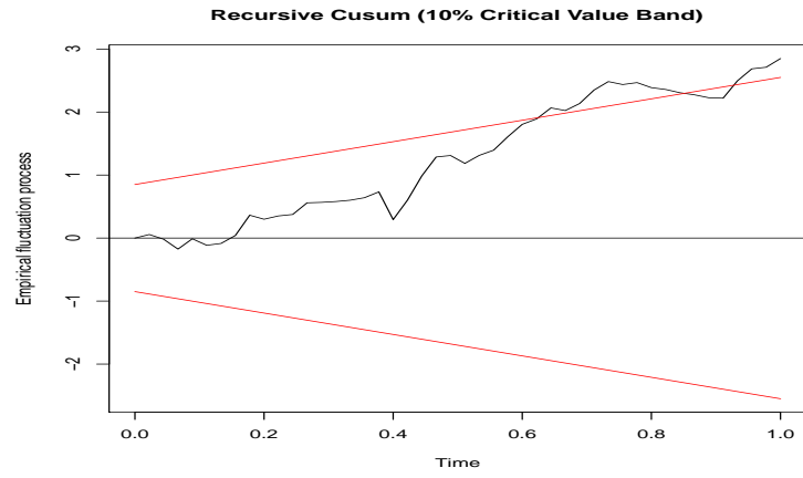
(a) Recursive CUMSUM Test
