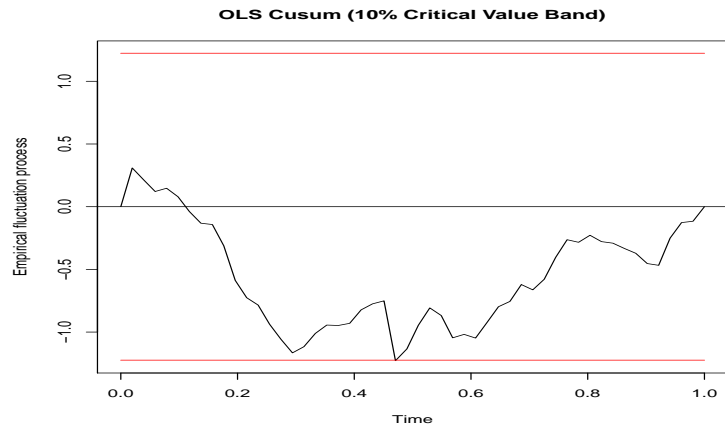
(b) OLS CUMSUM Test
