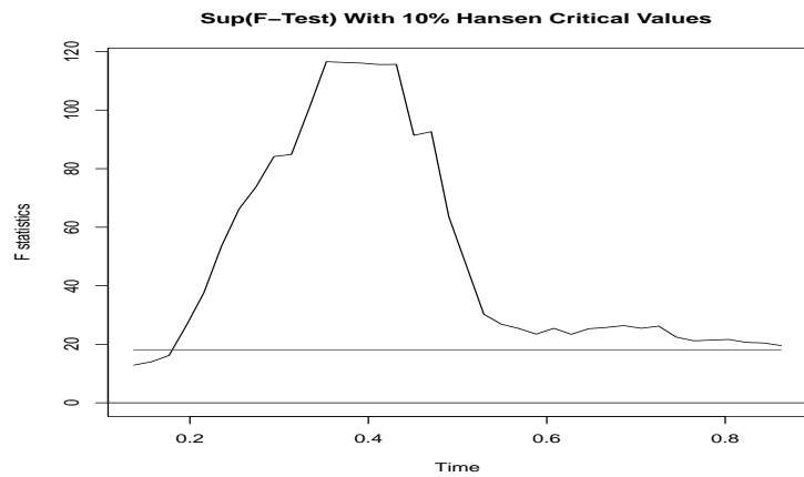
(c) Hansen's sup(F) Test
