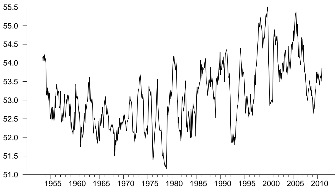
Figure 1a. Annual Average Raw Temperatures, CT_{t+12}
