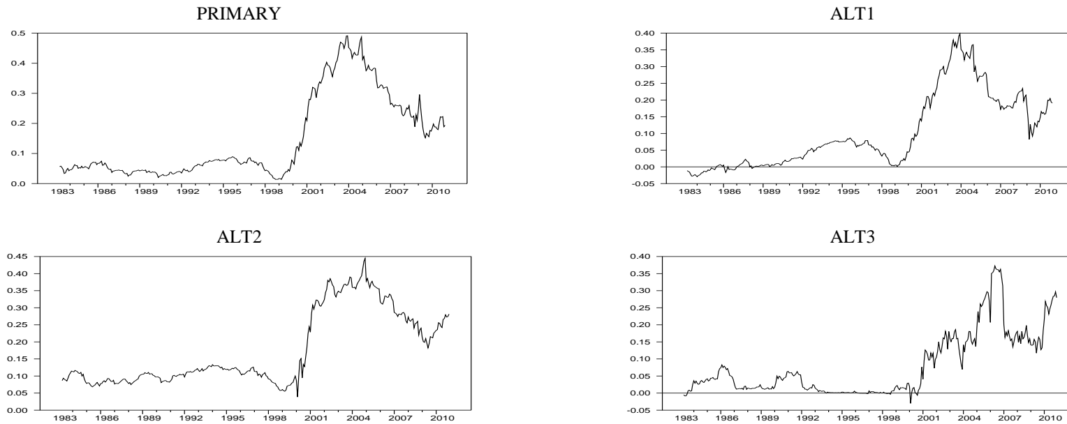
Figure 2. Rolling Impact Estimates of the Global-Warming Factor. The impact is estimated for the entire 1953:5 – 2010:12 sample using 30 years of data for each estimate. Accordingly, the first period starts in 1983:4. We update the estimates each month by dropping the earliest observation and adding the latest observation.
