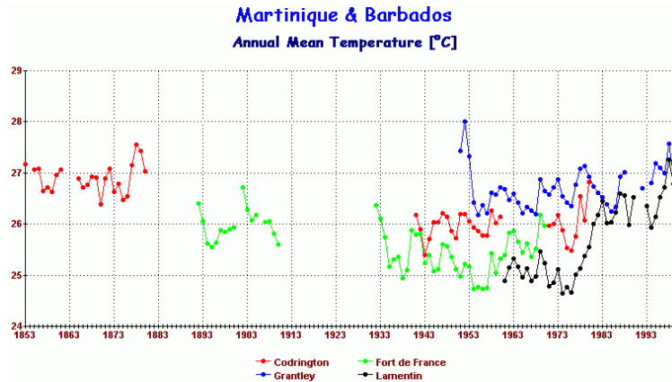
Figure 4: Annual Mean Temperature Four Reporting Stations, Martinique and Barbados
