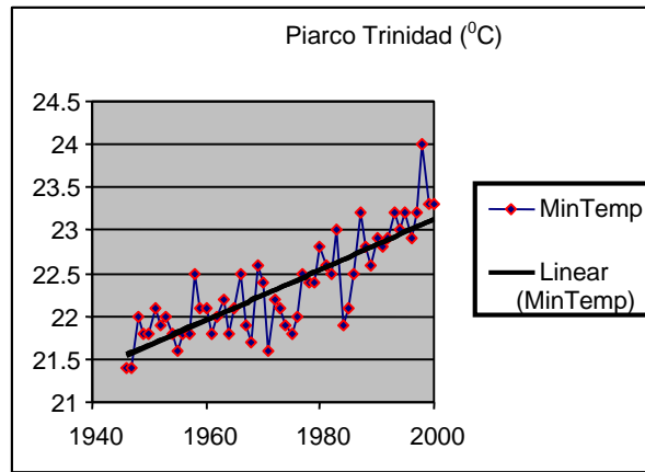
Figure 6: Annual Mean Minimum Temperature Piarco, Trinidad: 1946-2000
