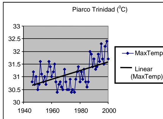
Figure 5: Annual Mean Maximum Temperature Piarco Airport, Trinidad: 1946-2000
