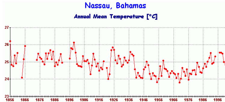
Figure 1: Annual Mean Temperature: Nassau, Bahamas
