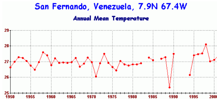
Figure 3: Annual Mean Temperature: San Fernando, Venezuela
