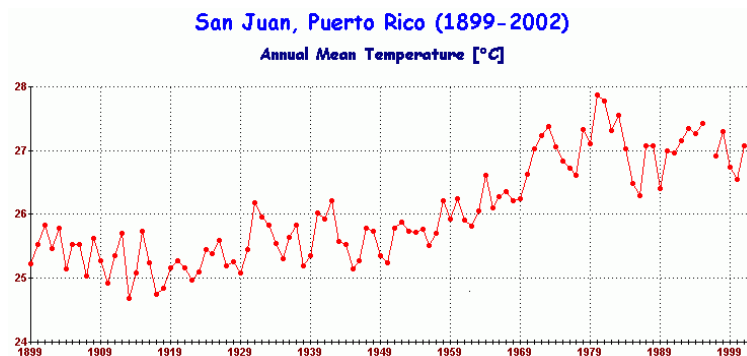
Figure 2: Annual Mean Temperature: San Juan, Puerto Rico (1899 – 2002)
