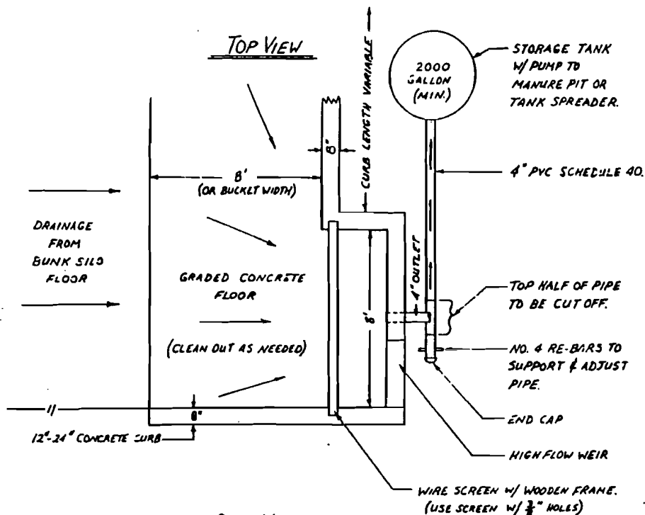
Figure 10. Low flow collection system (not to scale)
