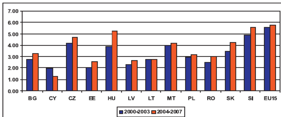
Figure 4: Yield of cereals in NMS (tonnes/ha)
