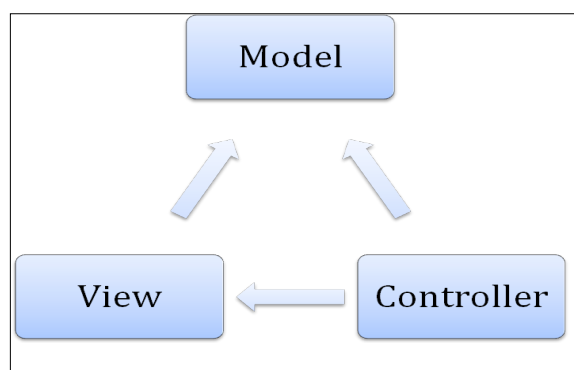
Figure 5: The principle of the MVC architecture (Microsoft, 2009).
