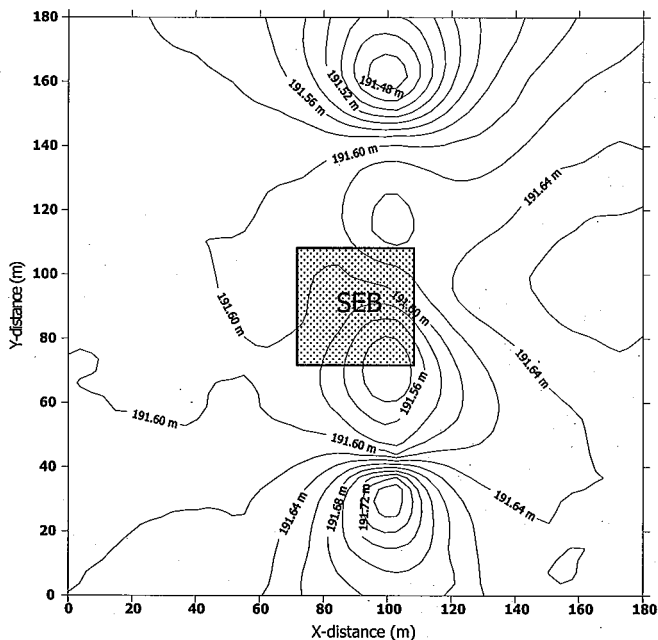
Figure 6 Groundwater levels during the first week of August 2000 (initial conditions).
