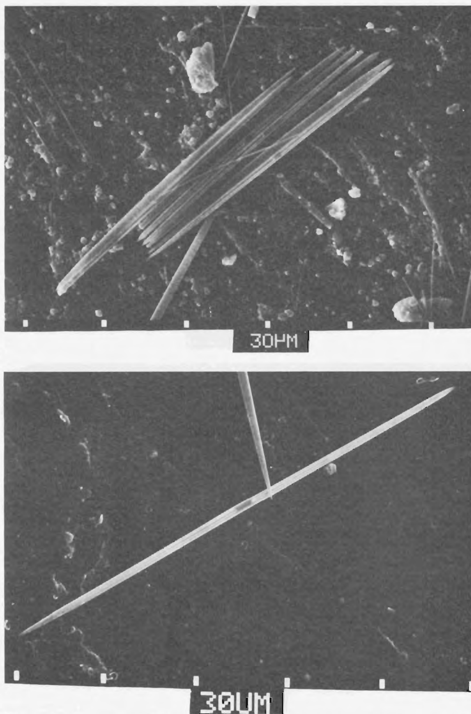
Fig. 5.2 (a) ( top ) Scanning electron micrograph of aligned calcium oxalate raphides from giant taro (cv Viagaga, Fiji), length about 100 \mu\text{m} , showing raphides that have a long tapering point at one end and an abrupt point at the other end. (b) ( bottom ) Single raphide, length 170 \mu\text{m} , of giant taro from Solomon Islands showing long tapering end, short abrupt end and a line down centre of the raphide.
