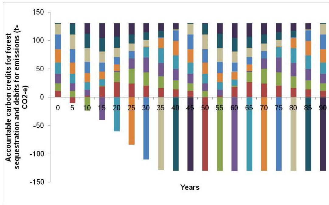
Figure 4: Carbon Credits (Sequestration) and Debits (Emissions) Over a Ninety Year Period for a Southern Natural Pine Forest Estate Managed on a Forty Year Rotation With Equal Areas in Each Age-Class
