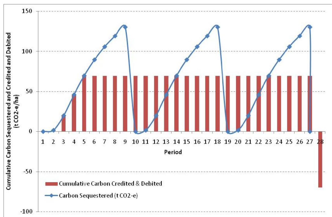
Figure 2: Above-Ground Carbon Sequestration Curve (blue), and Cumulative Carbon Credits Accrued to or Debited (red) per Hectare of Southern Natural Pine Forest Managed on a Forty Year Rotation under the Average Stock Approach
