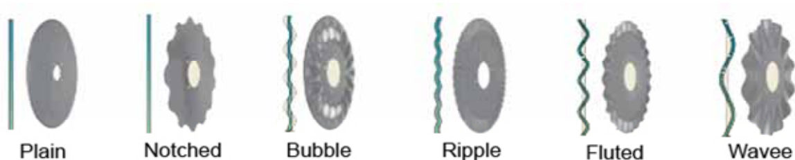
Figure 17: Typical cutting edge profiles for each general disc coulters type
