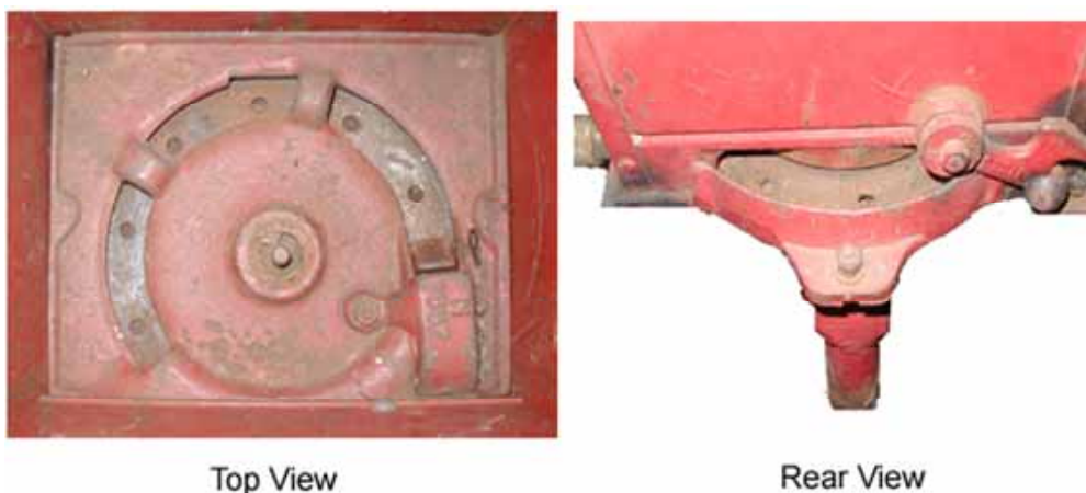
Figure 177: The top and rear views of a horizontal plate seed meter
