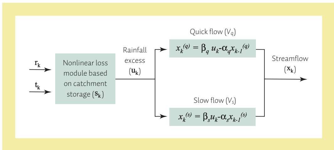
Figure 6.2 Generic structure of the IHACRES rainfall–run-off model. The climate inputs are rainfall ( r_k ) and temperature ( t_k ), though the temperature can be replaced by an estimate of the potential evaporation or potential evapotranspiration if this is available.
