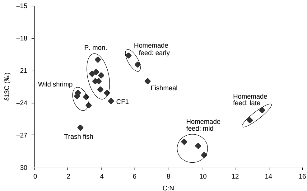
Figure 1. \delta^{13}\text{C} (‰) and C:N ratios for shrimp and feed at three farms in My Xuyen District. P. mon. = Penaeus monodon ; CF1 = commercial feed; early, mid and late denote times in the shrimp growth season.
