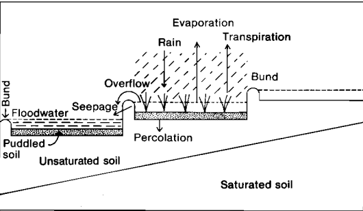
Fig. 3. Cross-section of a toposequence of banded fields, showing components of the water balance.
