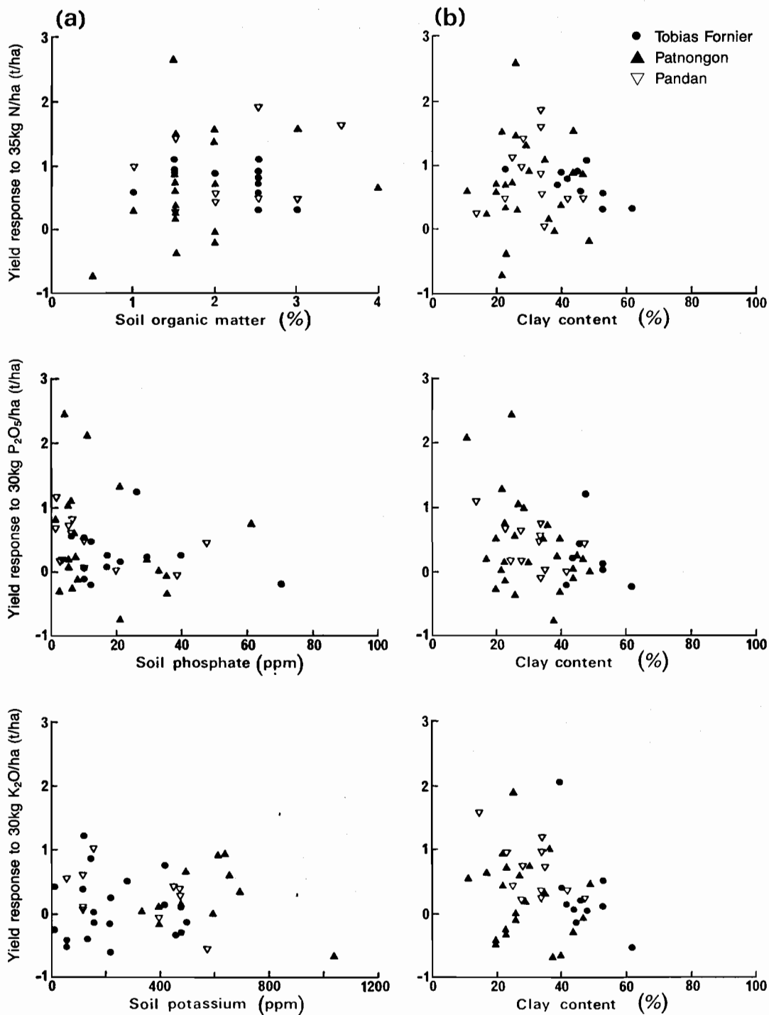
Fig. 4. Rice yield responses expressed in relation to soil tests: (a) responses to N, P and K fertilisers in relation to the levels of soil organic matter, available phosphate and potassium of the researcher-managed fields; (b) responses to N, P and K fertilisers in relation to clay content of the researcher-managed fields.
