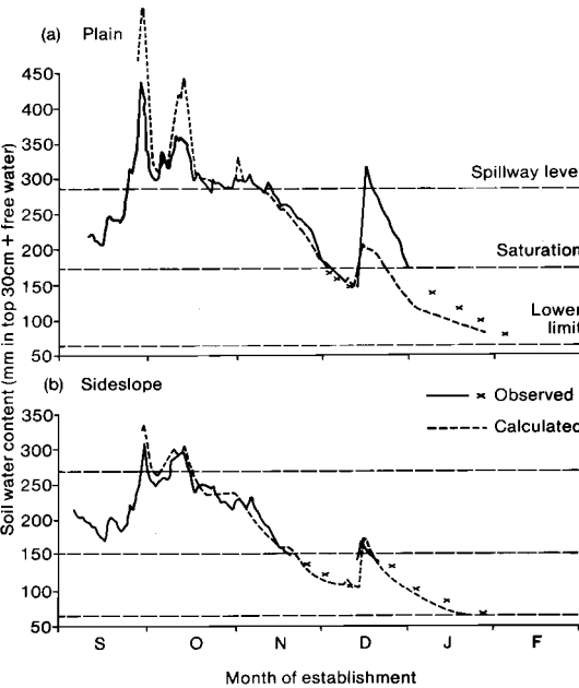
Fig. 4. Fit of the water balance model (dashed lines) to observations of soil water and standing water (solid lines and crosses) for two rainfed rice fields in Tigbauan, Iloilo. (a) plain position, (b) sideslope position. Observations are those of Bolton (1980).
