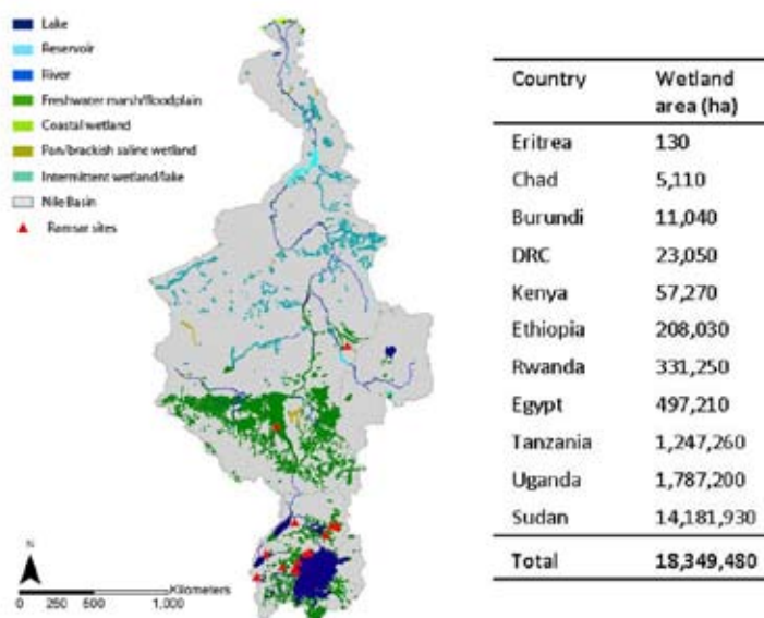
FIGURE 2. Spatial distribution and areal extent of wetlands within the Nile Basin. Data are derived from the Global Lakes and Wetlands Database (Source: Lehner and Döll 2004), and country-based Africover data sets (Source: Di Gregorio 2002).
