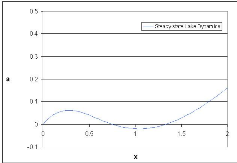
Figure 7: Lake Dynamics for b=0.48
