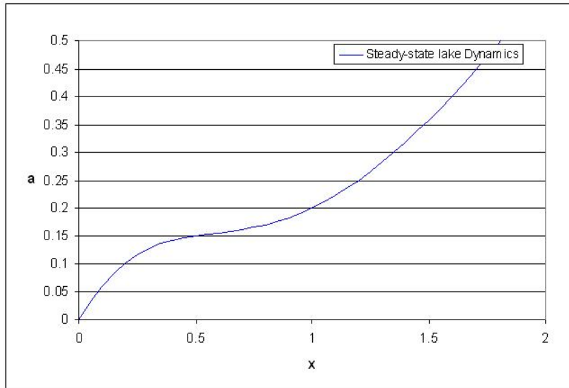
Figure 6: Lake Dynamics for b=0.7
