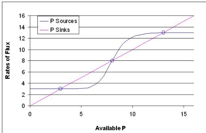
Figure 5: Phosphorous Sources and Sinks
