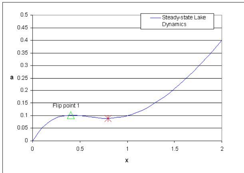
Figure 8: Lake Dynamics for b=0.6
