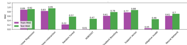
Figure 3. Models MAE for Rice Yield Prediction.
