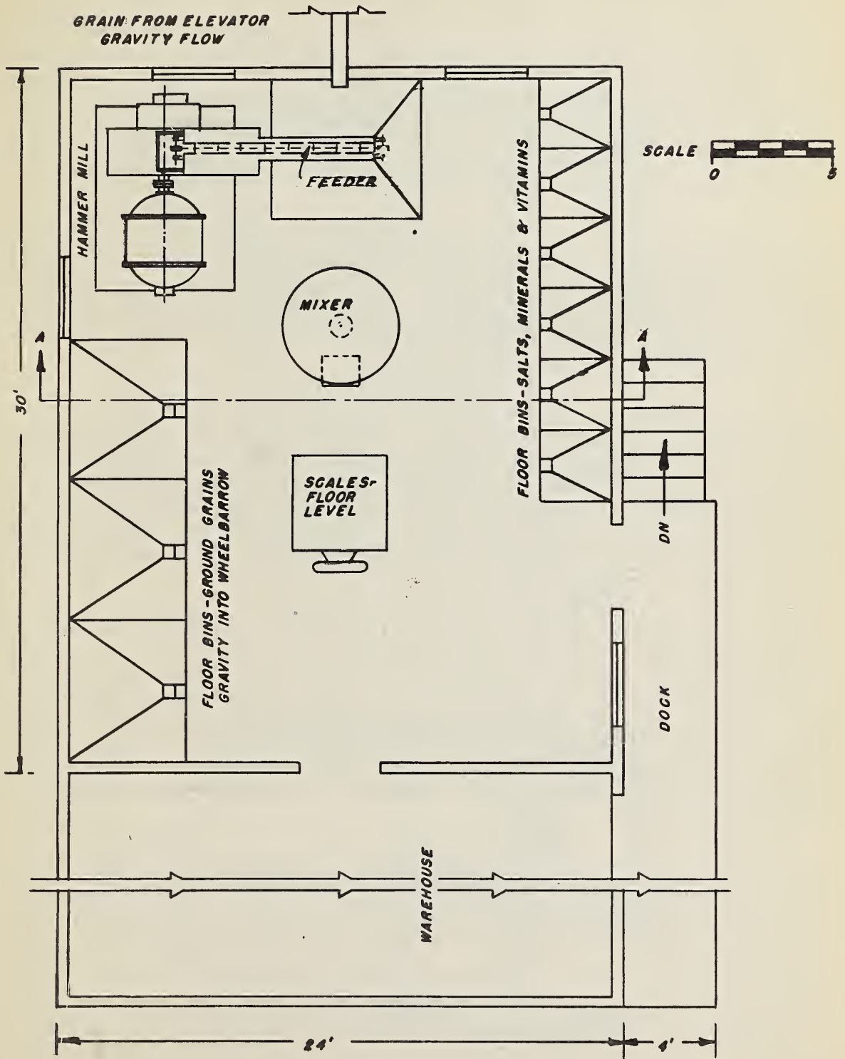
FIGURE 9 FEED MILL No. 2-ONE FLOOR WITH ADJACENT GRAIN STORAGE-FLOOR PLAN
