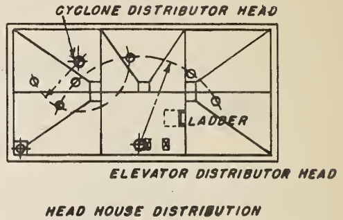
FIGURE 11 FEED MILL No. 3 - FLOOR PLANS OF MILL WITH ELEVATED BINS, HAMMER MILL PIT, AND ADJACENT GRAIN STORAGE - FLOOR PLANS -
