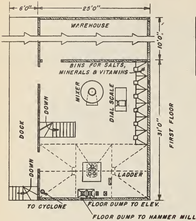
FIGURE 11 FEED MILL No. 3 - FLOOR PLANS OF MILL WITH ELEVATED BINS, HAMMER MILL PIT, AND ADJACENT GRAIN STORAGE - FLOOR PLANS -
