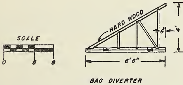
BAG DIVERTER
