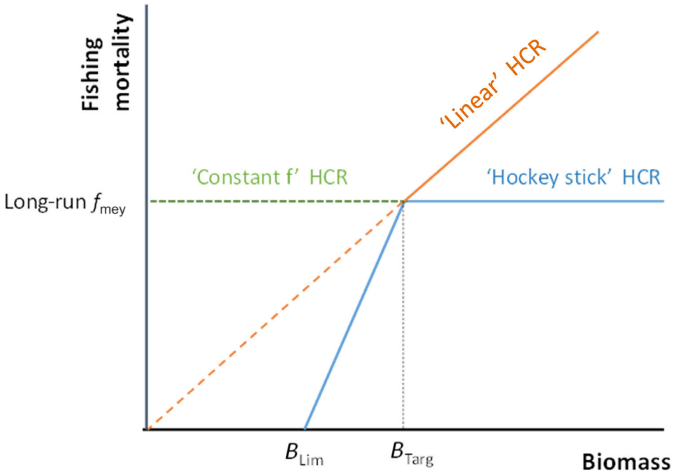
Figure 1 Alternative harvest control rules (HCRs) applied in simulations. For this study, B_{Targ} (the target biomass) was equal to B_{MEY} . B_{Lim} was assumed equal to 20 per cent of B_0 . [Colour figure can be viewed at wileyonlinelibrary.com ]
