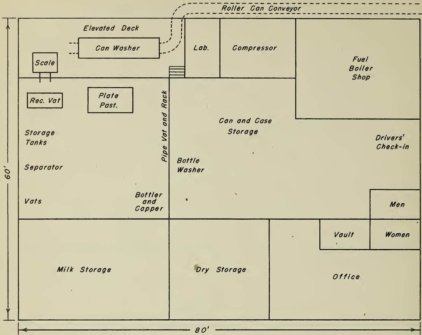
Figure 15. - Suggested floor plan for one-story pasteurizing plant, 3,000 gallons daily capacity.
