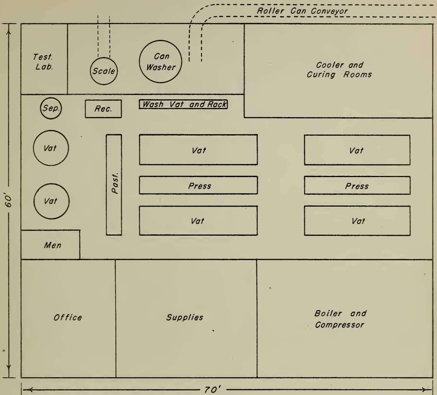
Figure 11. - Suggested floor plan for cheese plant of 40,000 pounds daily capacity.
