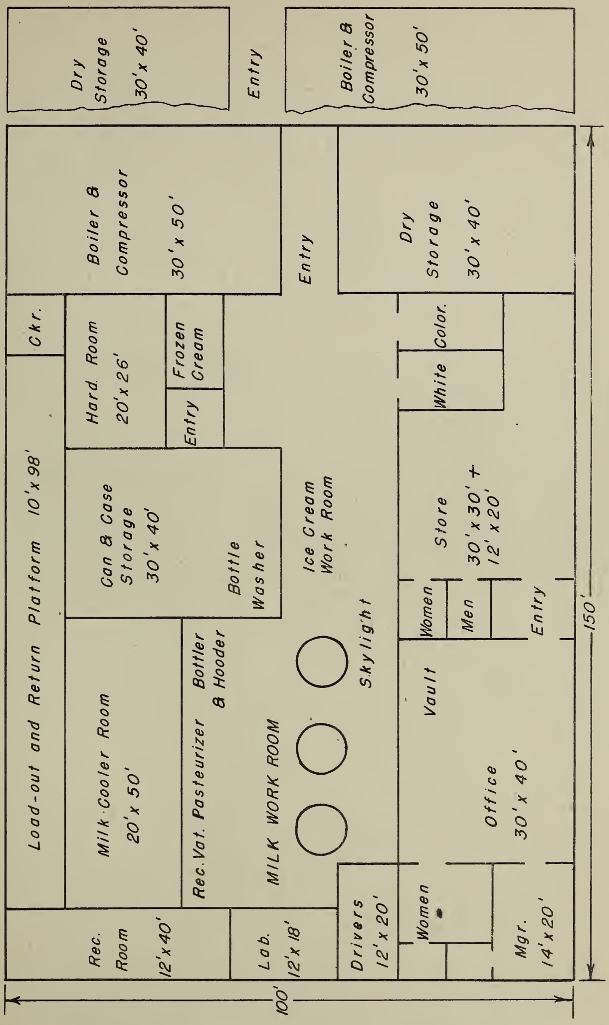
Figure 28. - Rearrangement of space in figure 27, of pasteurizing plant for over 5,000 gallons daily capacity.
