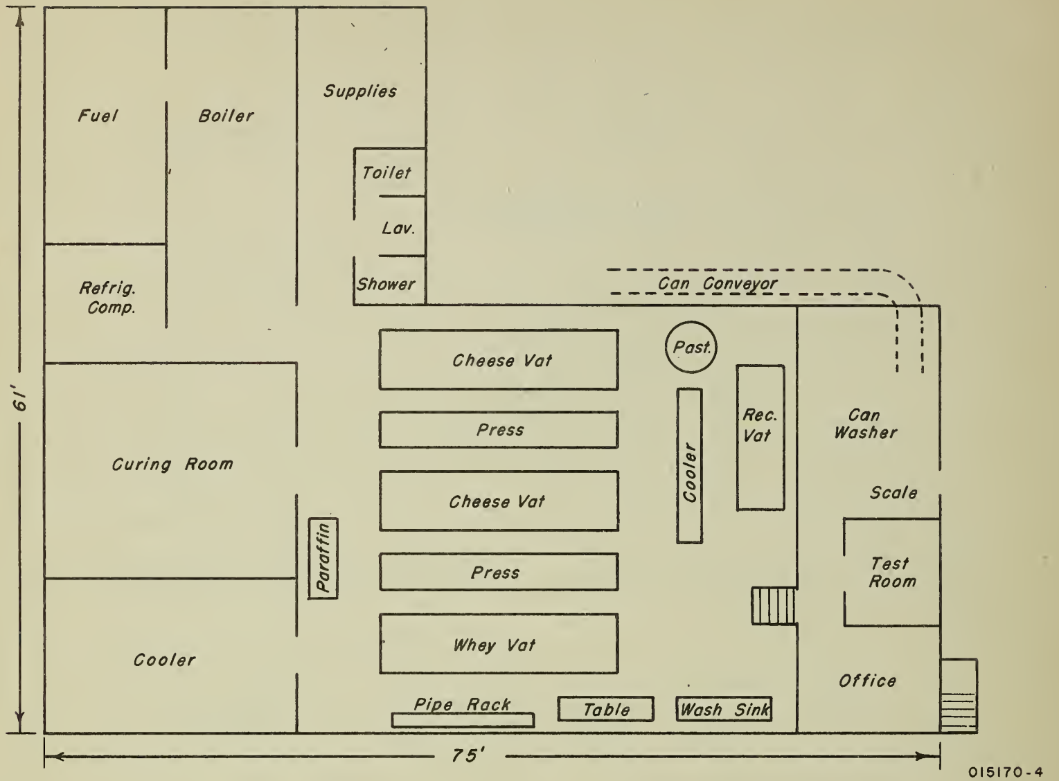
Figure 12. - Suggested floor plan for cheese plant.
