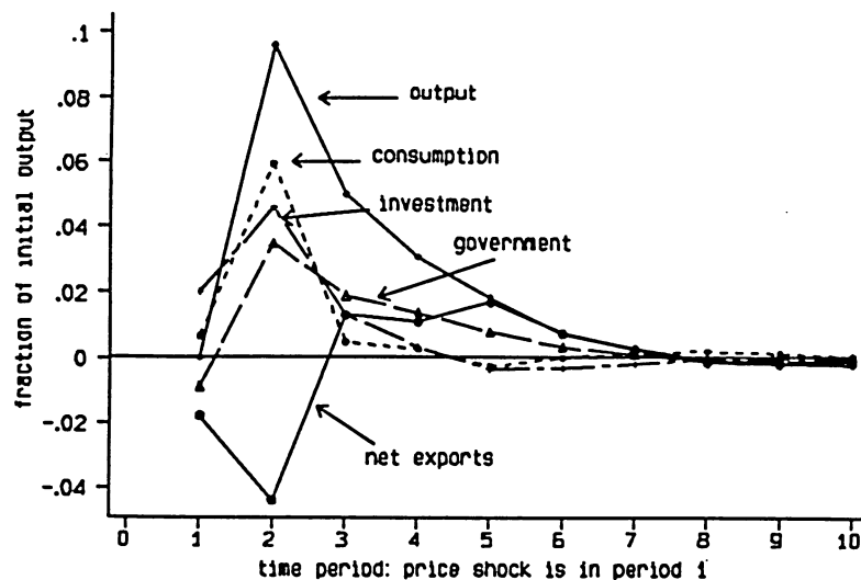
Figure 9: Impulse responses to a commodity price shock
