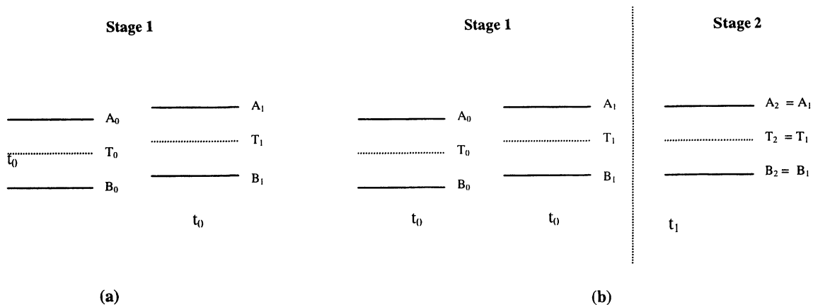
Fig. 3. The change in spread when the inventory levels is of no concern.
