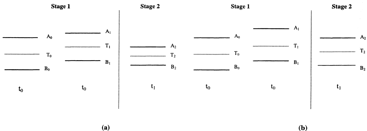
Fig. 4. Change in spread when there is excess inventory (a) During procurement (harvest) season (b) During off-season.
