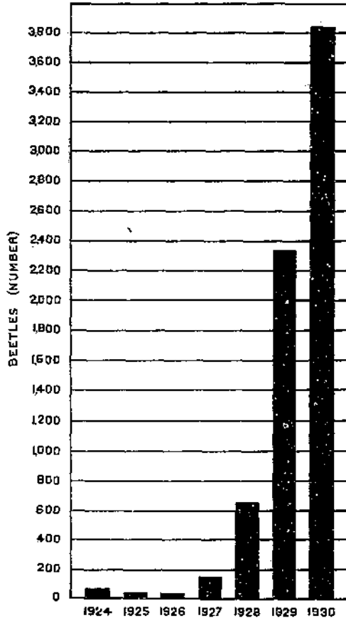
FIGURE 14.—Graph showing the maximum numbers of overwintered beetles on a 1/4-acre field in the foothills from 1924 to 1930, inclusive.
