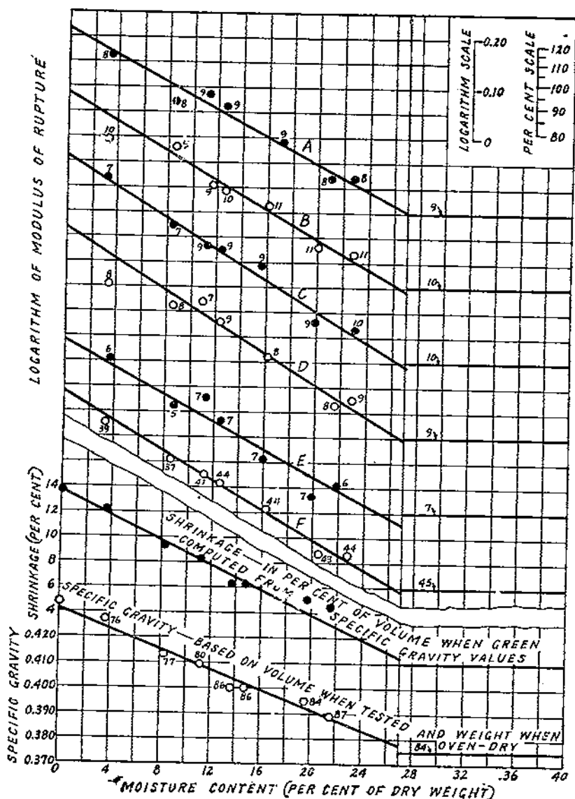
FIGURE 18.—Sitka spruce: Relation of average values of modulus of rupture by individual trees and of specific gravity and shrinkage in volume to moisture content. Numerals at points and on horizontal lines are numbers of tests averaged. Letters A to E each designate data for specimens from one tree. F is data for all trees combined and is identical with the modulus of rupture graph shown in Figure 14. For detailed data see Table 10
