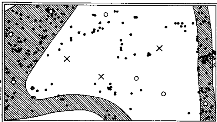
FIGURE 1.—Map of the study plot near Warrensburg, N. Y., which was logged in 1923. The haul roads that crossed the plot are shaded. The circles and black dots mark the location of the Ribes found on the plot in 1927, four years after the logging, the former representing the Ribes that were present on the plot in 1923 before the logging and the latter the Ribes plants that originated after the logging. The crosses mark the location of the three large hemlocks left by the loggers
