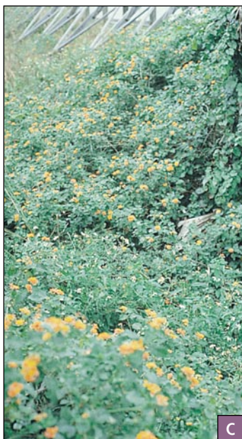
Figure 8. Lantana can grow in a wide range of habitats:
