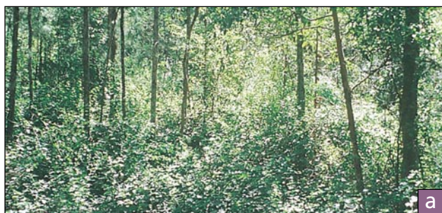
Figure 8. Lantana can grow in a wide range of habitats:
