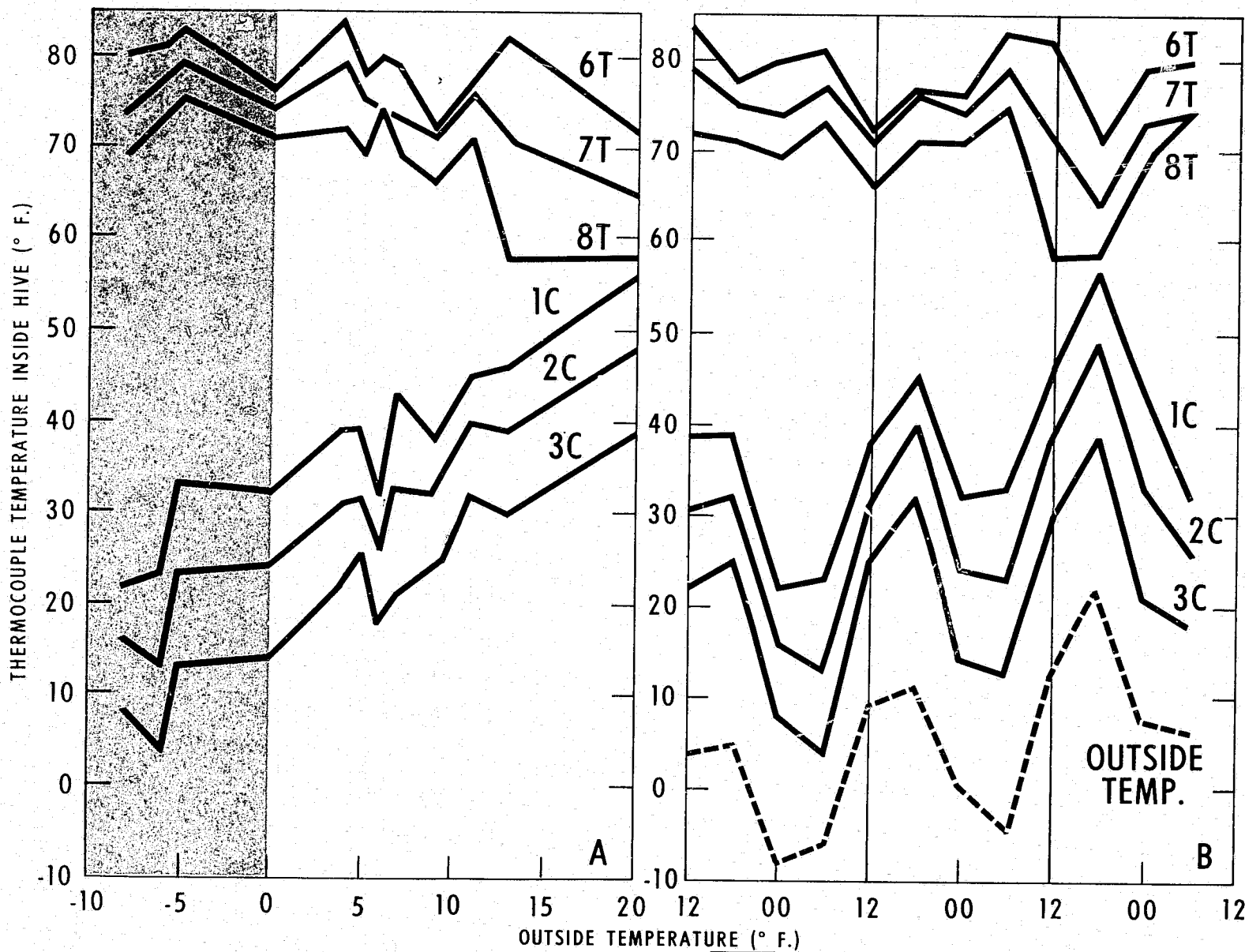
FIGURE 8.—Temperature variation in check colony versus outside temperature. (Thermocouple 8T is three-eighths inch above bottom edge of top body and 1C is one-fourth inch below top edge of center body; others are 1 inch apart in their respective directions.)
