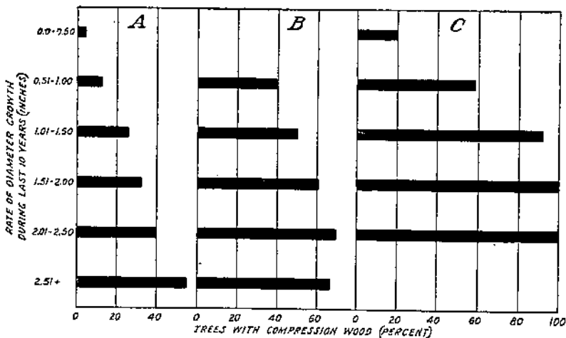
FIGURE 2.—Relationship of rate of diameter growth and various amounts of lean to percentage of trees having compression wood. Loblolly and longleaf pine, North Carolina and South Carolina: A, Slight lean; B, moderate lean; C, pronounced lean.
