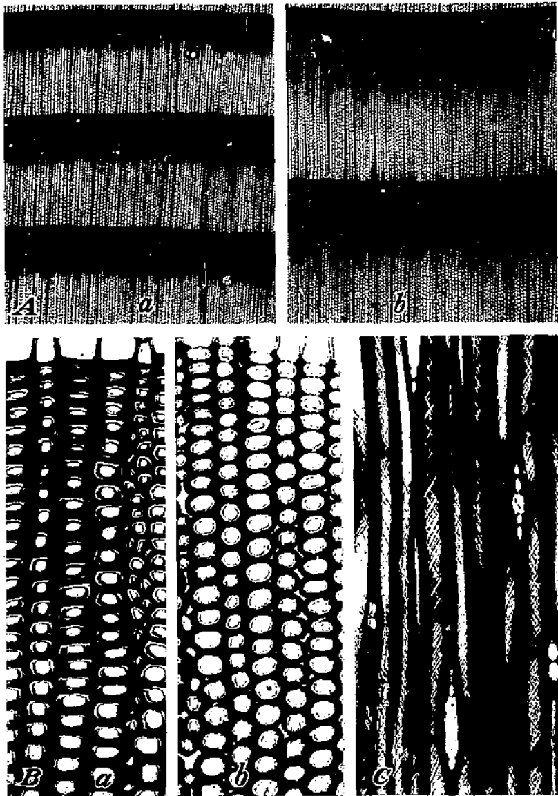
1. Transverse sections of Douglas fir: a , Normal wood showing relatively sharp demarcation between springwood and summerwood of the same annual ring in comparison with b , compression wood in which sharp demarcation is lacking. The darker horizontal bands are summerwood. Photomicrographs \times 20 . B , Transverse sections of Douglas fir showing typical summerwood cells of ( a ) normal wood and ( b ) compression wood. Note cracks in secondary cell walls, intercellular spaces, and circular cross-sectional shape of summerwood cells of compression wood. Photomicrographs \times 250 . C , Longitudinal section of Douglas fir showing typical summerwood cells of compression wood with spirally oriented cracks and striations in the secondary wall. Photomicrograph \times 250 .
