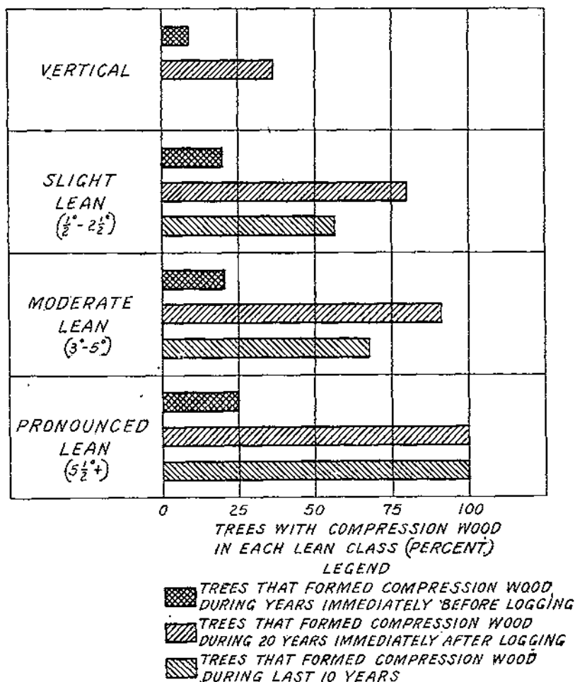
FIGURE 3.—Percentages of loblolly and longleaf pine trees by lean classes that had formed compression wood before and immediately after release by logging 20 years previously and during the last 10 years. Inclination determined just before felling.
