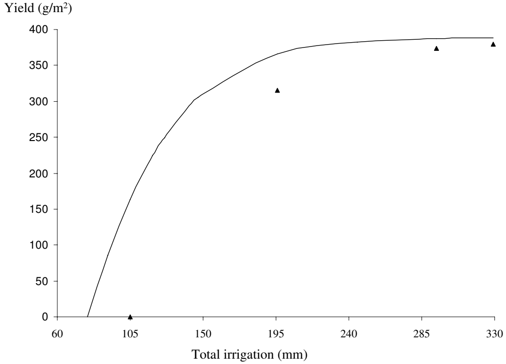
Figure 4: Loam water yield functions for Drip (solid line) and Flood (triangle symbols) vs. water allotment Q .
