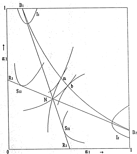
Figure 3 Two-Country Abatement Games
