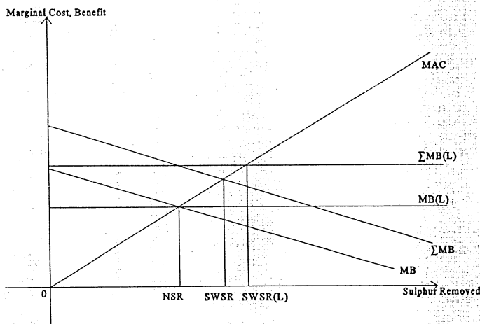
Figure 2 : Nash and SW Outcomes with Linear and Nonlinear Damage Functions
