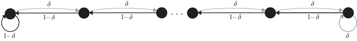
Figure 2: The unbalanced line, which demonstrates that a network may not converge to truth even if every agent's incoming trust is bounded. Agents are numbered from left to right.
